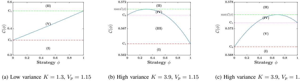
Fig. 2: Example plots of \mathcal{C}(\phi) , labeled with the ranges of C for which specific equilibrium regimes are possible, as defined in Theorem 1. These examples feature incumbent queuing parameters of \rho_{in} = 0.05 , \mu_{in} = 0.033 and K_{in} = 1.855 ; a customer traffic rate of \rho = 0.1 and service rate of \mu = 0.628 . We vary K and V_p to demonstrate different possible regions. Regimes (I) and (II) are always possible if C is set low or high enough. In the low variance ( K = 1.3 ) case, the monotone increasing nature of \mathcal{C}(\phi) results in Regime (V) being the only other possibility. In the high variance ( K = 3.9 ) case, the unimodal nature of \mathcal{C}(\phi) results in a region where regime (IV) predominates, alongside either (III) or (V) depending on which of C_0 or C_1 is the minimum value of the function; this will be determined by V_p in conjunction with the other parameters.
