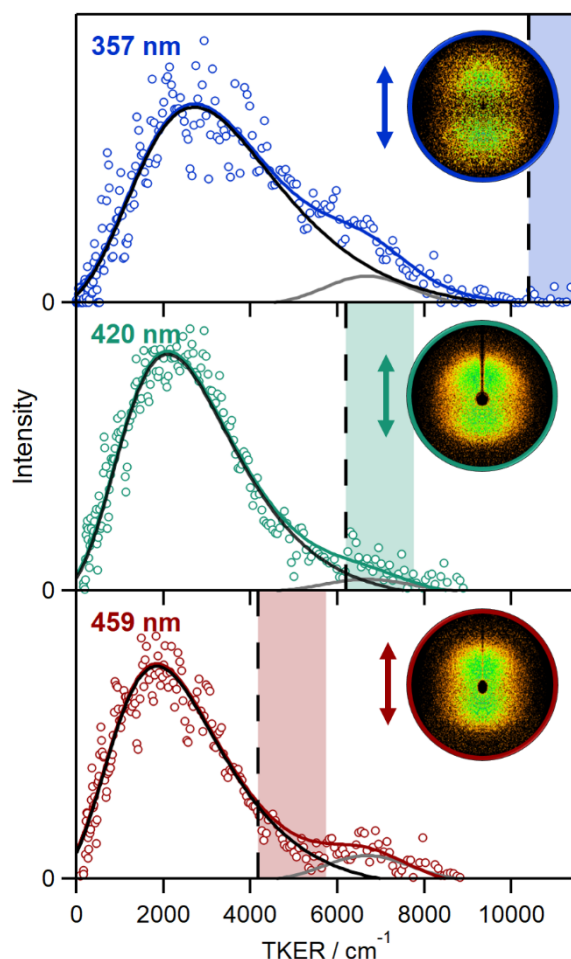
Figure 5. Total kinetic energy release (TKER) distributions (open circles) and the fits (colored lines) obtained by velocity map imaging of O ( 1 D) products following UV-vis excitation at 357 nm (upper), 420 nm (middle), and 459 nm (lower). In each panel, a weak IO component (gray curves) arising from incomplete background subtraction is fit with Gaussian distribution centered at 6680 cm -1 . The TKER distributions for the O ( 1 D) + 2-butenal (S 0 ) product channel are well represented by Gumbel distributions (black lines). The vertical black dashed lines indicate the energy available (E avl ) to products for the cZE conformer of 2-butenal oxide at each UV-vis wavelength with the shaded region indicating E avl for less stable conformers. Insets are the corresponding raw images of the O ( 1 D) photoproducts. The double-sided arrows represent the polarization of the UV-vis radiation.
