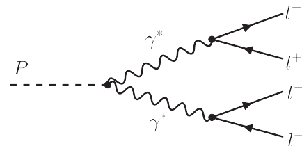
FIG. 1. Feynman diagram of pseudoscalar decays into four leptons, known as double-Dalitz decays.
