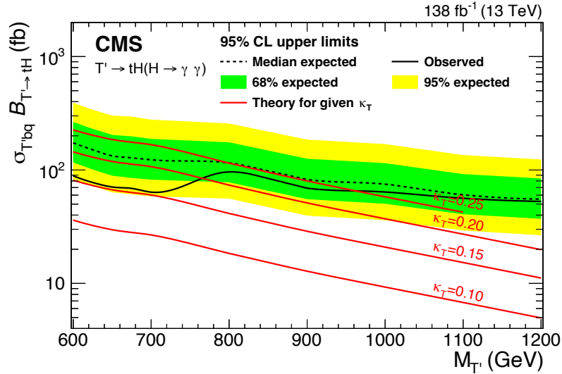
Figure 4: The combined, leptonic plus hadronic, expected (dotted black) and observed (solid black) upper limits at 95% CL on \sigma_{T'bq} \mathcal{B}_{T' \rightarrow tH} are displayed as a function of M_{T'} . The green (yellow) band represents the 68% (95%) of the limit values expected under the background-only hypothesis. The theoretical cross sections for the singlet T' production with representative \kappa_{T'} -values fixed at 0.1, 0.15, 0.2 and 0.25 (for \Gamma/M_{T'} < 5\% ) are shown as red lines.
