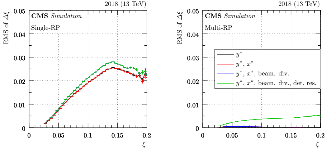
Figure 36: Example of resolution studies for \tilde{\zeta} (2018 pre-TS1, sector 56). On the vertical axes, \Delta\tilde{\zeta} refers to the difference between the reconstructed and simulated \tilde{\zeta} . On the horizontal axes, \tilde{\zeta} denotes the simulated value. The different colors refer to different smearing effects considered. Black: only vertical vertex smearing, red: in addition also horizontal vertex smearing, blue: in addition also beam divergence, green (the most complete scenario): in addition also detector spatial resolution. The error bars represent statistical uncertainties. Note that some curves are superimposed. Left: single-RP, right: multi-RP reconstruction.
