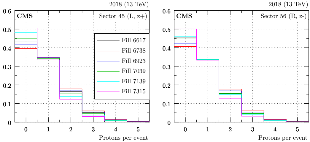
Figure 29: Multiplicity of reconstructed protons per arm and per event (2018 data). The histograms are normalised to unit area. Different colors correspond to different fills as indicated in the legend. Left: sector 45, right: sector 56.
