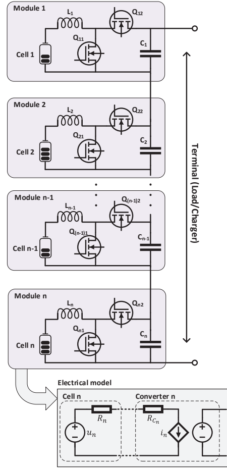
Fig. 1: The circuit structure of large-scale BESS.
