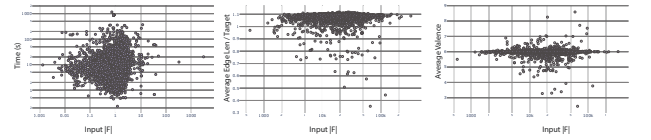
Fig. 13. Timings, target edge length ratio, and valence for every model in the dataset. Most models finish within a minute. The target edge length ratio measures how well our algorithm simplifies the meshes to reach the desired edge length, with an optimal value of 1. Since uniform remeshing strives to generate regular meshes, for most models our algorithm is able to obtain the optimal valence of 6.
