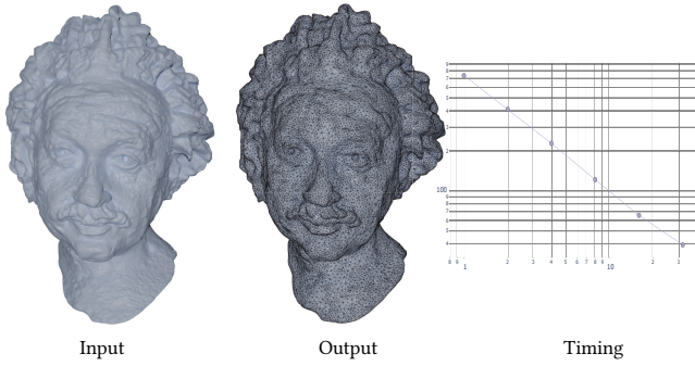
Fig. 11. Shortest edge collapse with envelope containment of a model with 857, 976 faces. Our method successfully generates a mesh with 71, 298 faces in 37.49s with 32 threads (731.32s serial, 725.34s on a single thread, speedup of 20×).
