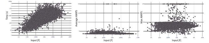
Fig. 14. Timing, max and average AMIPS energy (capped at 20) for maximum 25 iterations of tetrahedral meshing. Most models finish withing 20 minutes with only a few taking up to a day. Even by limiting the iterations to 25, most models reach an average AMIPS energy lower than 10, with optimal value at 3.
