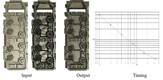
Fig. 12. Uniform remeshing with envelope containment check of a model with 198, 918 faces. Our method produces a mesh with 68, 202 faces in 29.11s with 32 threads and 493.54s for a single thread (483.68s for the serial version) leading to a speedup of 16×.
