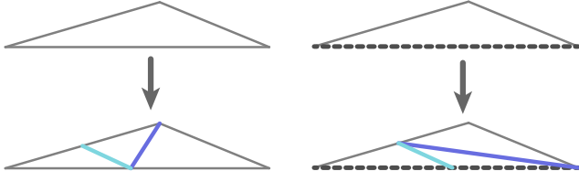
Fig. 10. Example of splitting the longest edge on the bottom of the triangle. On the left, the bottom edge can be split first with the introduction of the dark blue edge; next, the left edge is split (added the light blue edge) leading to a decreasing maximum edge-length. On the right, the bottom edge is locked (illustrated by a dashed line); when the bottom edge is unlocked in the next iteration, the edge length decrease is less effective.
