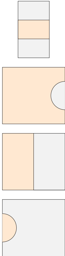
Fig. 4. Equilibrium shapes in any dimensions, depending on the proportion of the lighter versus the heavier fluid: orange stands for the lighter fluid, while gray stands for the heavier fluid
