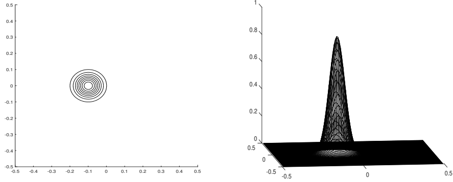
Figure 1: \mathbb{E}(c_{MC})(x, T) solved under h=1/128 and \Delta t=\pi/64 from the view of top (left) and side (right).
