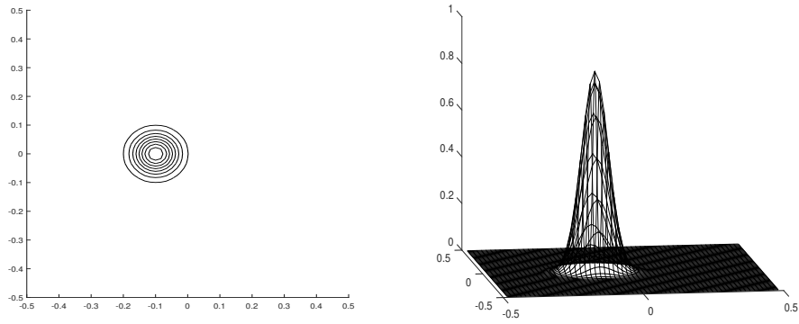
Figure 2: \mathbb{E}(c_h^{N_t})(x) solved under h=1/60 , \Delta t=\pi/64 and N=2 from the view of top (left) and side (right).
