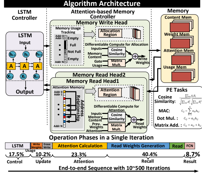
Fig. 2. Differentiable Neural Computer Algorithm.
