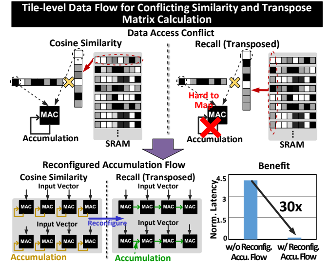
Fig. 5. Reconfigured dataflow for tile-level conflicts.
