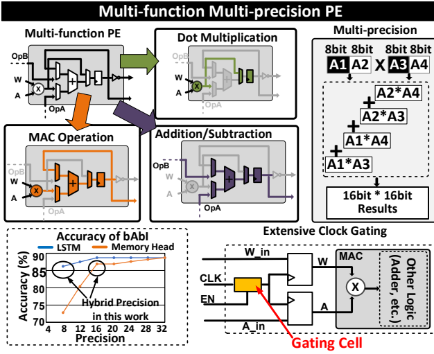
Fig. 6. PE Reconfiguration, multi-precision, clock-gating.
