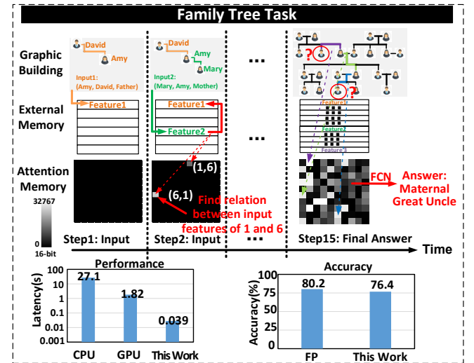
Fig. 9. Detailed demonstration of family tree task.
