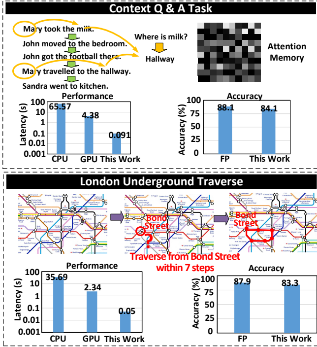
Fig. 10. Details of Q&A task and London underground traversal task.
