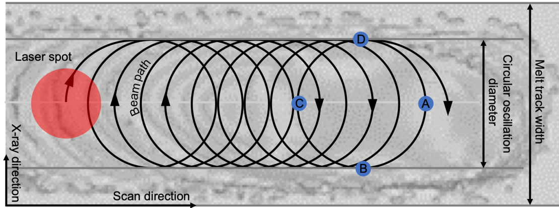
Fig. 1 Laser oscillation schematic. A schematic of a circular oscillation superimposed on a linear laser scan path highlighting the key dimensions and positions during the periodic laser movement.
