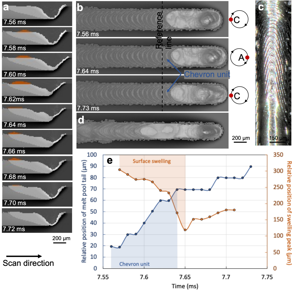
Fig. 4 The formation of chevron pattern. The centerline cross-sectional views of a simulated oscillating melt track (400 W laser power and 400 mm \text{s}^{-1} laser scan speed with 0.12 mm circular oscillation diameter) in a show the formation of the surface swelling which is highlighted in orange and the corresponding top-down views in b show the formation a chevron unit. A comparison in d shows a no-oscillation case with the same laser parameters. The optical image
