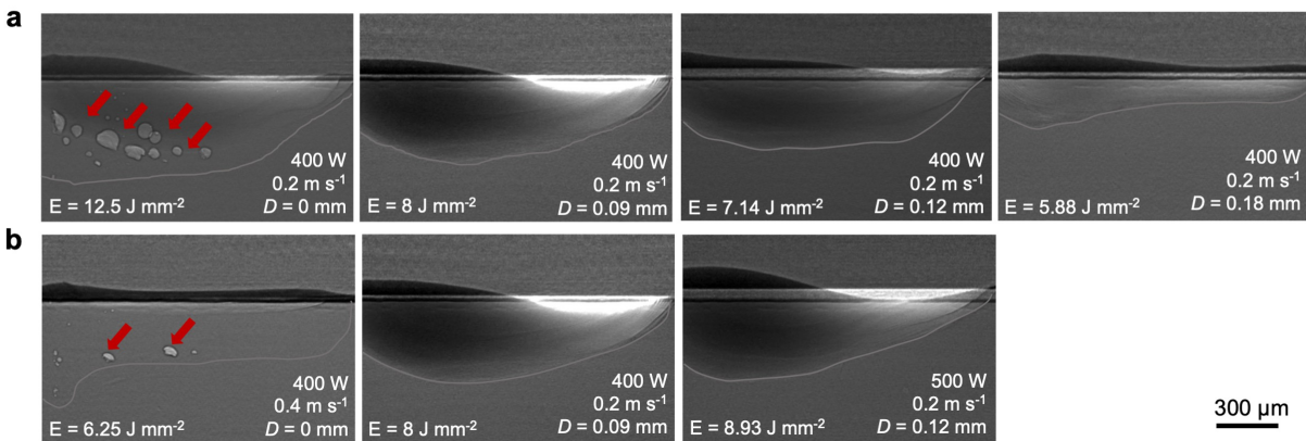
Fig. 8 X-ray images of solidified melt tracks. The DXR images of the post-solidified melt track showing the porosity reduction induced by a increasing the laser oscillation from 0 mm to 0.18 mm at laser power of 400 \text{ W} and speed of 0.2 \text{ m s}^{-1} and b introducing laser oscillation to
