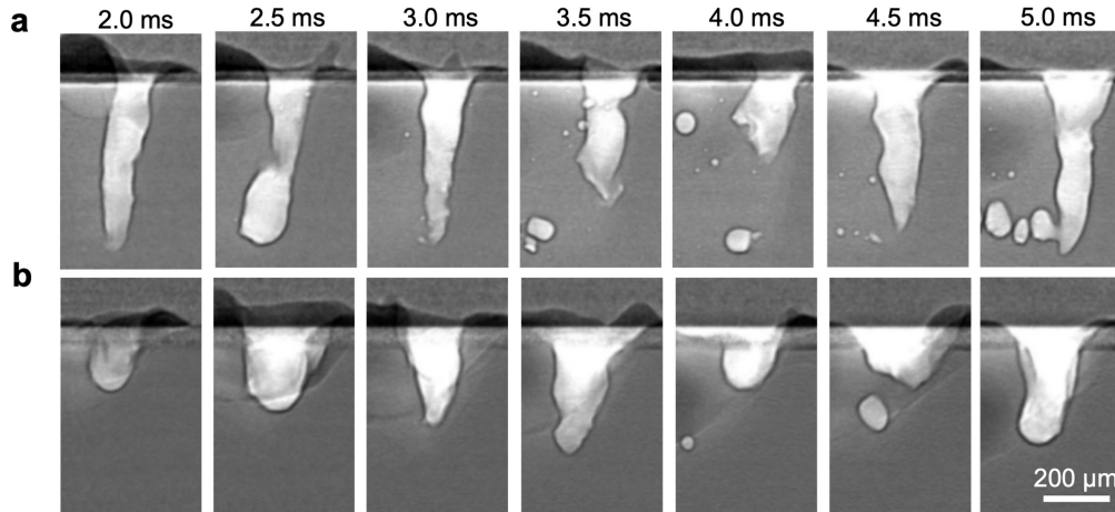
Fig. 6 Keyhole porosity mitigation due to laser oscillation. DXR images capturing the keyhole depth evolution. The top series a shows the keyhole evolution in the case of linear scan and the bottom series b shows the corresponding case with circular oscillation diameter of 0.12 mm. Both scans used 400 W laser power and 0.2 \text{ m s}^{-1} scan speed. Note the timestamp shows the elapsed time since the laser was triggered. (See Supplementary Movies 05, 06.)
