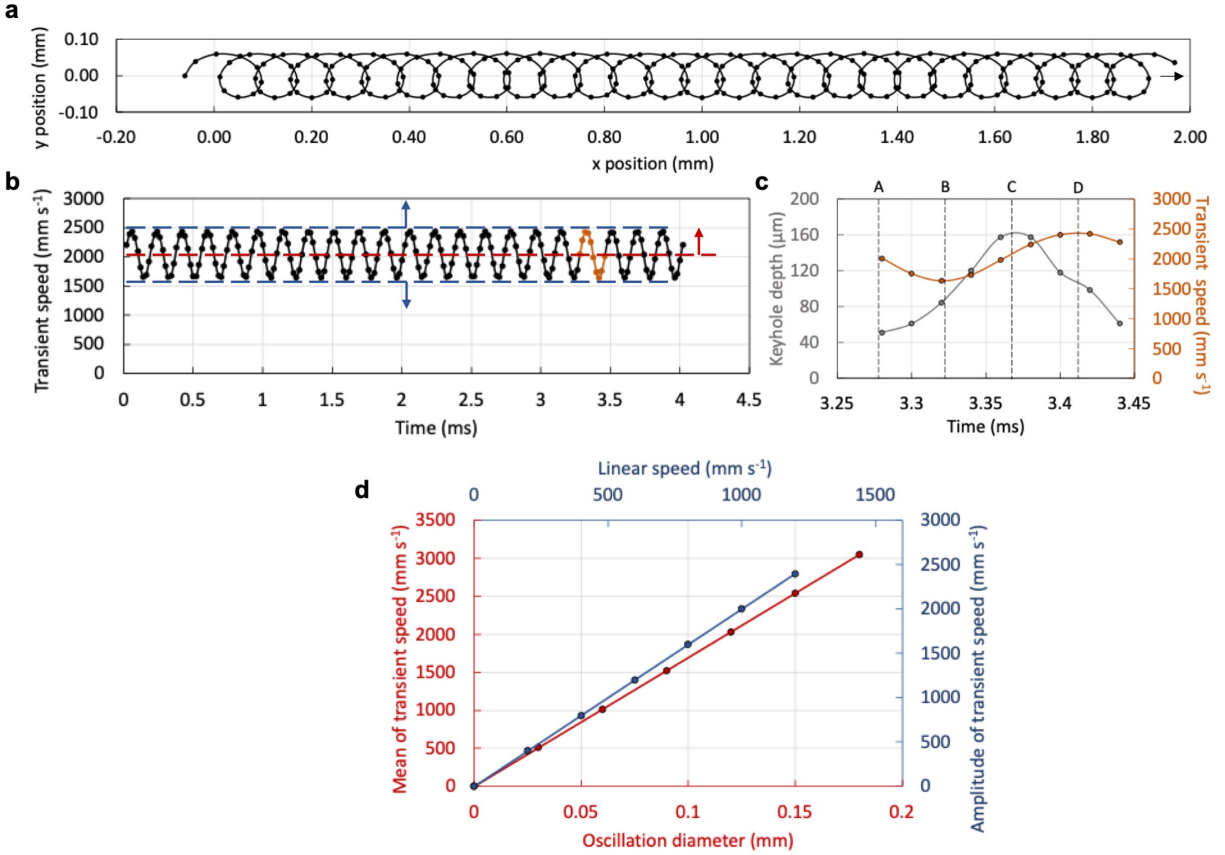
Fig. 2 Laser oscillation path and quantification. a Laser scan path, b calculated transient speed, and c calculated transient speed and experimental keyhole depth profile of an oscillation cycle between 3.28 ms and 3.44 ms of an experiment with process parameters of 400 W, 400 \text{mm s}^{-1} linear scan speed, and 0.12 mm circular oscillation diameter. Note that the corresponding DXR video frames can be found in Fig. 3a. The blue and the red arrows in b highlight the response of the transient speed profile to the increasing linear scan speed and the increasing oscillation diameter, which is also summarized in d .
