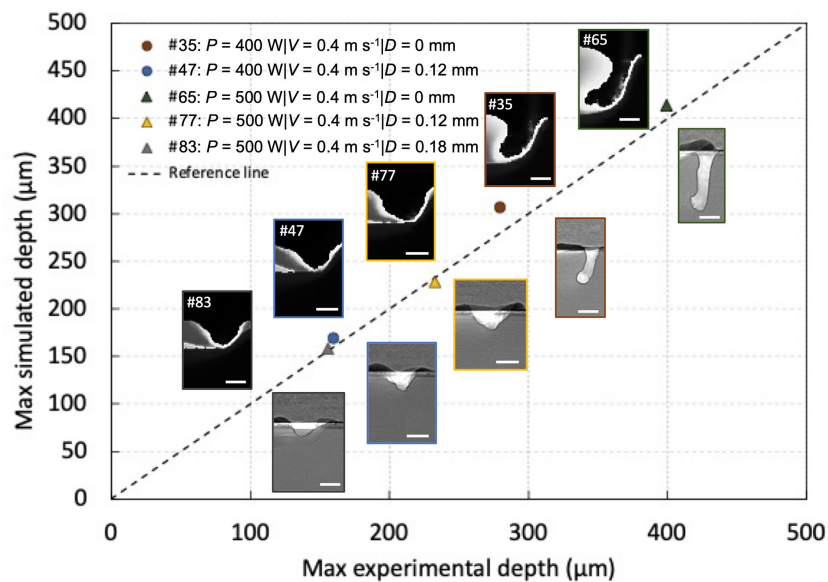
Fig. 7 Keyhole morphology comparison between the simulations and the experiments.
