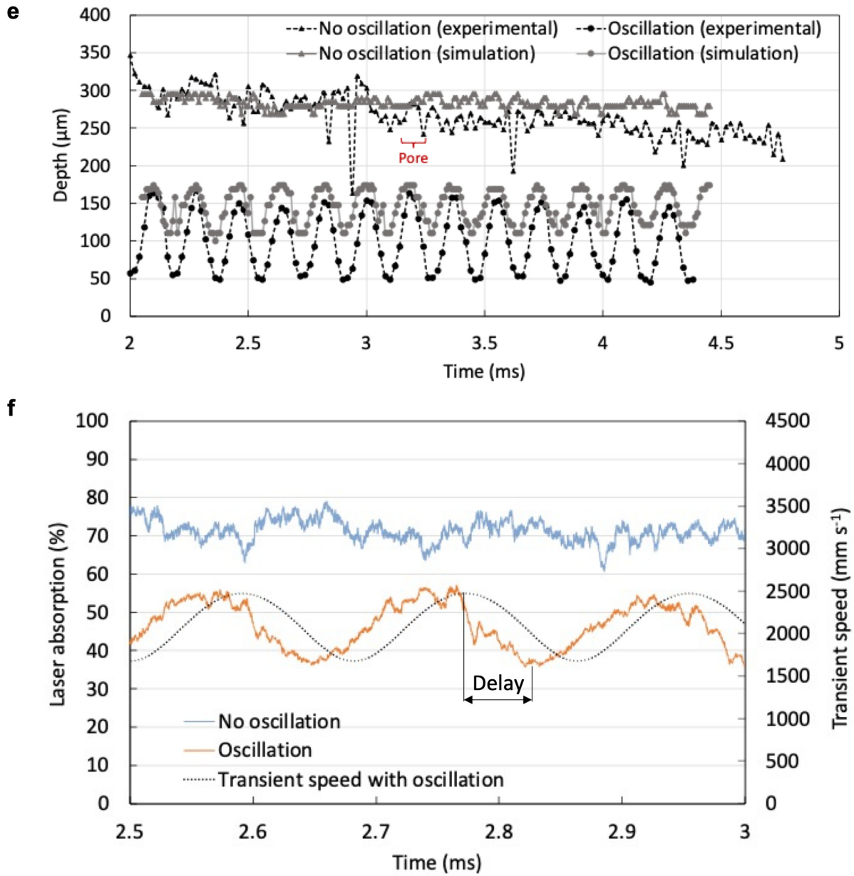
Fig. 3 Comparison of an oscillating keyhole and a non-oscillating keyhole. DXR video frames revealing the keyhole geometries in the experiments and the corresponding simulations at 400 W laser power and 400 \text{mm s}^{-1} laser scan speed with a, b 0.12 mm circular oscillation diameter and c, d no oscillation. Note that the timestamp at each frame is the accumulated time since the laser was triggered. The sequences in a, b are also labeled with the respective positions, A, B, C, D, of an oscillation unit. The green color (no temperature dependence) on the sample indicates the melted/solidified part of the track and the green color in the keyhole cavity represents the traced rays. The corresponding keyhole depth profiles are shown in e and the corresponding laser absorption profiles for both the simulated oscillation and linear cases calculated from the traced rays are shown in f . (See Supplementary Movies 01 - 04.)
