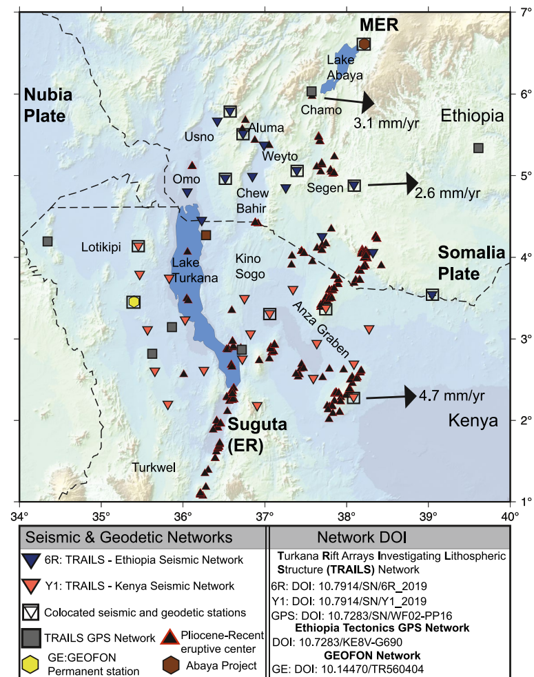
Figure 3. Inverted triangles are the Turkana Rift Array to Investigate Lithospheric Structure (TRAILS) project seismic stations (Ebinger (2018) Y1 network = orange; Bastow (2019) 6R network = blue. Other seismic networks (GEOFON Data Center (1993) = yellow hexagon; Ogden et al. (2021) network = brown hexagon). Gray square boxes show the spatial distribution of 12 continuous and eight campaign Global Navigation Satellite System (GNSS) stations. GNSS and seismic stations that are colocated have seismic stations overlain with a black box. Black arrows indicate plate motion in mm/yr relative to the fixed Nubia plate (after Kogan et al., 2012; Knappe et al., 2020). Note that 2.6 mm/yr velocity in southern MER is an underestimation of velocity due to the lack of GNSS stations in South Sudan (Figure S2 in Supporting Information S1). Pliocene-Recent eruptive centers are black triangles with red outline (after Global Volcanism Program, 2013; Sullivan, 2023).
