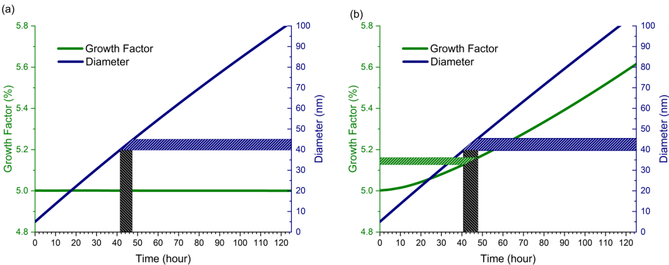
Figure 1: Growth factor and diameter vs. time for dry (no ALW) ammonium sulphate seed particles with an initial diameter of 5 nm. (a) Condensation of NVOCs and partitioning of SVOCs only. (b) SVOC 0 DIMER formation in addition to condensation and partitioning.
