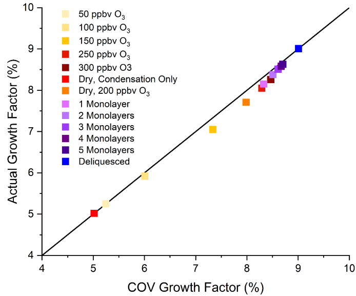
Figure 5: COV Growth Factor obtained from outlet minus inlet diameter change vs. Actual Growth Factor (average of GFs within the flow tube for each simulation in Section 4). Colours correspond to those shown for the simulations in Figures 3 and 4. The line shows a 1:1 ratio.
