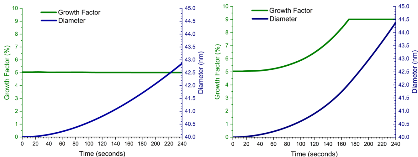
Figure 2: Growth factor and particle diameter vs. time for 40 nm dia. ammonium sulphate seed particles traveling through the flow tube, growing by (a) condensation of NVOC and partitioning of SVOC alone, and (b) with SVOC 0 DIMER formation included.
