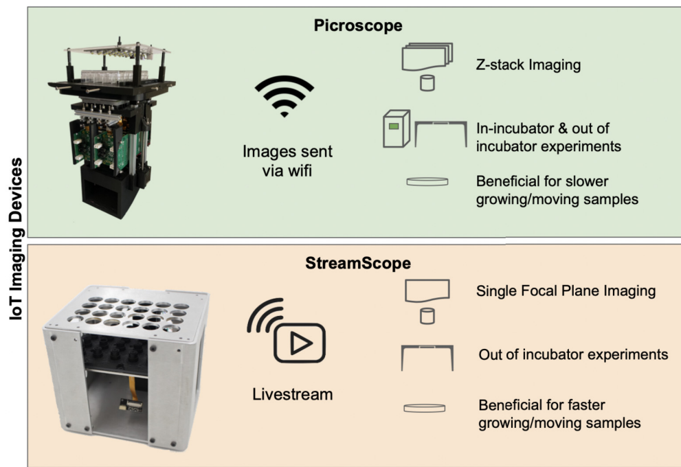
Fig. 1. Comparison of remote imaging devices 2 different remote imaging platforms were used, the Picroscope collects z-stack image data inside an incubator while the Streamscope livestreams a view of a sample on a lab bench.
