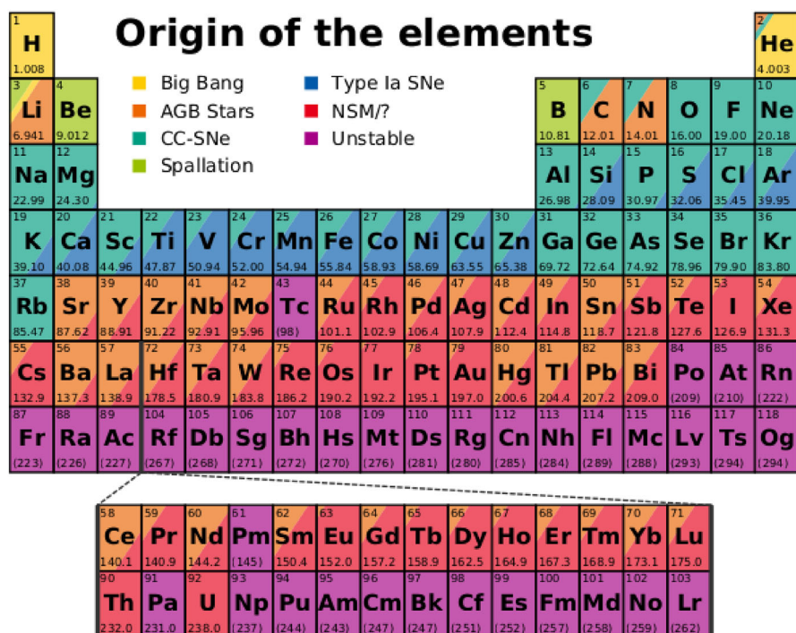
Fig. 37 The periodic table of the elements, where the processes of the preceding figure are translated into stellar sites. It should be noticed that the s - and r -process should be divided into weak and main components, where the weak components are related to different sites than indicated in the plot, like massive stars for the weak s -process and probably rare classes of supernovae for the weak r -process. Image courtesy of M. Reichert
