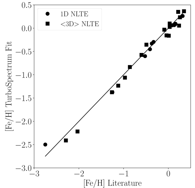
Fig. 8. [Fe/H] determined from the Turbospectrum fit versus values from the literature (see text). For the TS fit, the adopted value is the \langle 3D \rangle NLTE fit, or the 1D NLTE fit in cases where a \langle 3D \rangle NLTE fit was not available.
