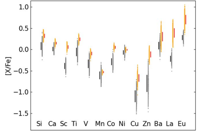
Figure 2. [\text{X}/\text{Fe}] ratios derived by Mucciarelli et al. (2021; see Table 1) for NGC 2005 (gray points) and the other five LMC globular clusters (orange dots), respectively. Each [\text{X}/\text{Fe}] ratio is represented by 1000 points following a Gaussian distribution. For the seek of the reader we included the corresponding 1\sigma error bars represented by black and red segments, respectively.
