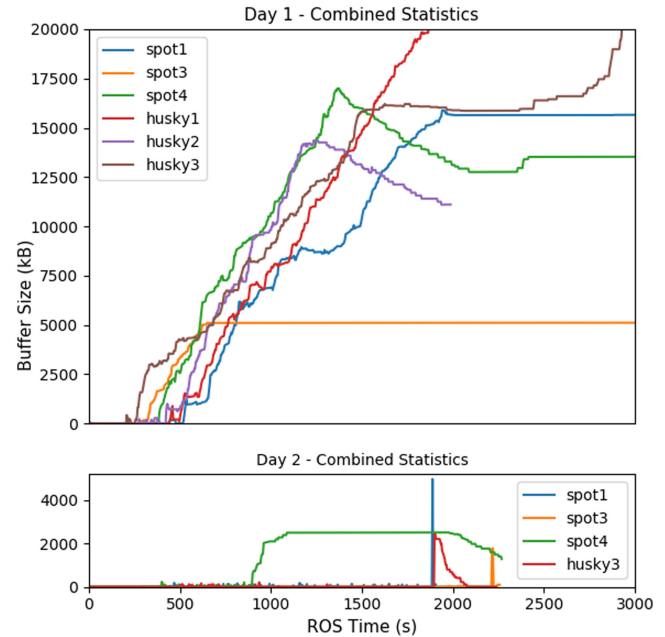
Fig. 8. Size of the data reporter buffer (summed over all key and mission-critical topics). The top graph depicts results from Day 1 with the data classification from CHORD and the bottom graph depicts results from Day 2 with the new data classification.
