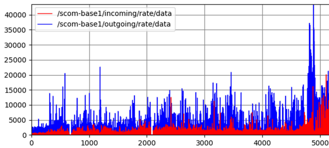
Fig. 7. KY Underground data rates (kbps) received by the base station (red) and transmitted by the base station (blue). Robots actively explore from 1019 to 4609 sec. After exploration ended, as the robots returned to the base, the data rates increased.
