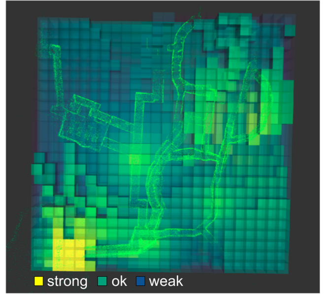
Fig. 4. Connectivity map of the DARPA SubT Finals competition environment based on predicted signal strength, which can inform autonomy and augment situational awareness for the human supervisor.
