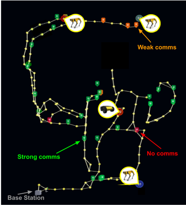
Fig. 3. Information RoadMap (IRM) constructed collaboratively during exploration of the DARPA SubT Finals competition environment. The environment state is indicated by green, orange, and red comms checkpoints which represent strong, weak, and no comms, respectively.
