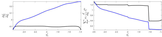
Fig. 6: left: the optimal direction \frac{q'_2}{q'_1} (in blue) and an erroneous demonstration (in black) for the lateral raise exercise; right: instantaneous penalty for the direction basis objective functions of the PSM and erroneous demonstration. Here, i indexes all direction basis objective functions.
