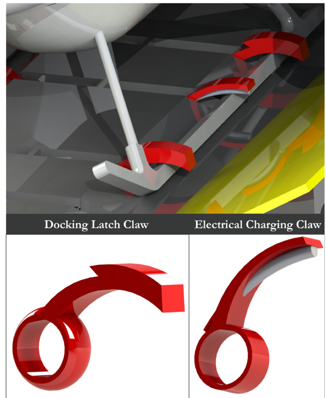
Figure 3: Top Row: MiniHawk VTOL secured to Docking & Recharging Backpack. Bottom Row: i) Docking Claw with increased material at the area that contacts the skids. Increased material reduces the amount of flex in that particular region of the part. ii) Electrical Charging Claw with conductive wire.
