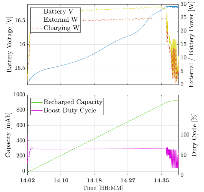
Figure 5: Externally-powered recharging of the MiniHawk VTOL by the DRB. Top row: MiniHawk battery voltage and input & battery recharging power. Bottom row: MiniHawk battery recharged capacity and Power Management Stack boost conversion duty cycle.
