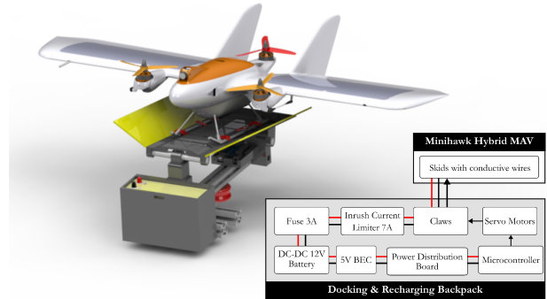
Figure 2: Docking & Recharging Backpack design overview. Detail: Subsystems Block Diagram.
