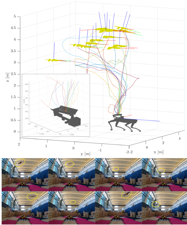
Figure 4: Top row: Reliability validation of the passive docking process during aggressive landing approaches, through a motion-captured experimental study. Bottom row: Indicative instances of the landing repeatability experiments inside the motion capture space.
