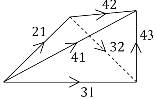
FIG. 6: A negatively oriented tetrahedron. The 3-cocycle assigned to it is \omega^{-1}(g_{43}, g_{32}, g_{21}) .
