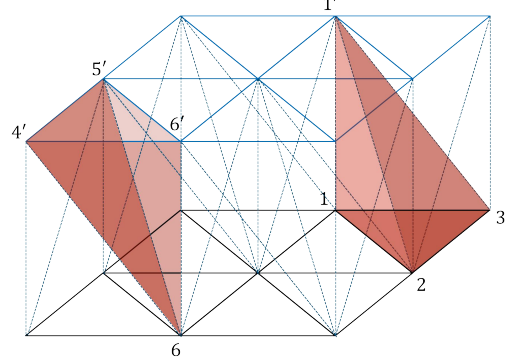
FIG. 2: The phase factor \text{Amp}(\{g_v\}, x) can be given by the triangulation of such prisms, where g_{v'} = g_v x .
