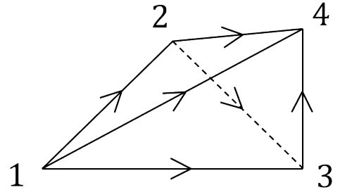
FIG. 3: A positively oriented tetrahedron. The 3-cocycle assigned to it is \omega(g_4 g_3^{-1}, g_3 g_2^{-1}, g_2 g_1^{-1}) .
