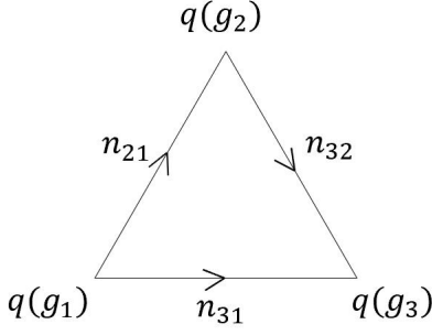
FIG. 13: One plaquette on a triangulated lattice.
