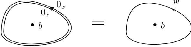
FIG. 17: The operator (H^x_{\partial R})^2 applying on curve \partial R is equivalent to the braiding phase between the g -flux of an anyon b ( g is the holonomy along \partial R ), and the charge of the anyon \omega .
