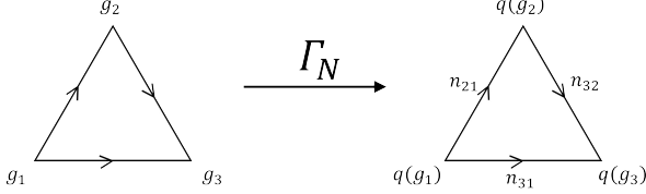
FIG. 7: The gauging map \Gamma_N maps the normal part from vertex DOFs to edge DOFs.
