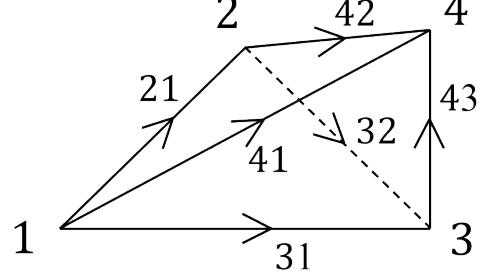
FIG. 9: A negatively oriented tetrahedron. The 3-cocycle assigned to it is \omega^{-1}(g_4 h_{43} g_3^{-1}, g_3 h_{32} g_2^{-1}, g_2 h_{21} g_1^{-1}) .
