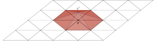
FIG. 5: The phase \tilde{W}_v^g is defined as the multiplication of the phases corresponding to the tetrahedrons. Here, g_{v'v} = g .
