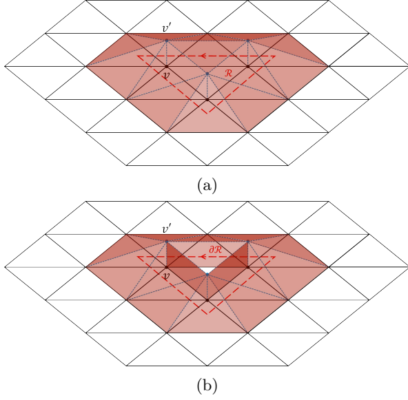
FIG. 15: (a) Symmetry action inside of region \mathcal{R} “lifts” \mathcal{R} such that all the simplex in the region correspond to \tilde{\omega} . (b) This symmetry action can be equivalently regarded as the insertion of symmetry branch line on \partial\mathcal{R} .
