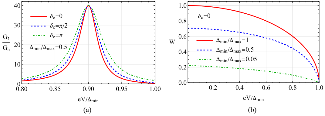
FIG. 3. (a) Normalized conductance as a function of bias voltage for several values of \delta_c at \epsilon_\uparrow = 0.9 \Delta_{\min} as indicated by the horizontal dashed line in Fig. 2(b). (b) Weight of the peaks in the conductance W , see Eqs. (22), (27), and (34), as a function of bias voltage for several values of \Delta_{\min}/\Delta_{\max} . In all panels, we assume a circular Fermi surface, consider tunneling into a high-symmetry point, and use the s + d_{x^2-y^2} gap \Delta(\varphi) = (\Delta_{\max} + \Delta_{\min})/2 + (\Delta_{\max} - \Delta_{\min}) \cos(2\varphi)/2 ; we fix G_n/G_Q = 0.05 in (a) and \delta_c = 0 in (b).
