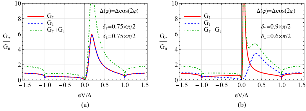
FIG. 5. Differential conductance as a function of voltage bias for several values of the scattering phases. (a) Spin-independent scattering \delta_\uparrow = \delta_\downarrow = 0.75\pi/2 leads to a single spin-polarized peak in (G_\uparrow + G_\downarrow)/G_n . (b) The peak is split by adding a spin-dependent scattering phase with \delta_\uparrow = 0.9\pi/2 and \delta_\downarrow = 0.6\pi/2 . Solid red and dashed blue lines correspond to spin-up ( G_\uparrow/G_n ) and spin-down ( G_\downarrow/G_n ) conductances, respectively. Dash-dotted green lines denote the conductance summed over spin projections (G_\uparrow + G_\downarrow)/G_n . In both panels, we assume a circular Fermi surface, use the d -wave gap \Delta(\mathbf{k}) = \Delta \cos(2\varphi) , and consider tunneling into a high-symmetry point.
