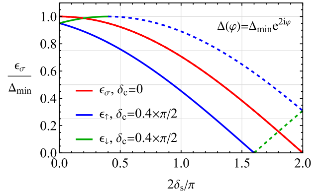
FIG. 6. Normalized energy of the subgap states \epsilon_\sigma / \Delta_{\min} as a function of \delta_s for \delta_c = 0 (red line) and \delta_c = 0.4\pi/2 (blue and green lines). The presence of spin-dependent scattering splits the spin-degenerate level (red line) into two states \epsilon_\uparrow (blue line) and \epsilon_\downarrow (green line) at \delta_s \leq \delta_c . The bound states have the same spin polarization for \delta_s \geq \delta_c . Solid and dashed lines show two different branches of bound states with the same spin polarization, see \epsilon_\uparrow^p and \epsilon_\uparrow^h in Eq. (C1). We assume a circular Fermi surface (parametrized by the angle \varphi ), consider tunneling into a high-symmetry point, and use the d_{x^2-y^2} + id_{xy} gap \Delta(\varphi) = \Delta_{\min} e^{2i\varphi} .
