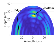
Fig. 8. Range-angle profile
