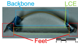
Fig. 4. Robot Structure
