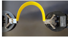
Fig. 5. Instron testbed
