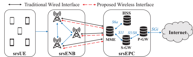
Fig. 1: Diagram of the traditional srsRAN architecture with wired interface (black solid lines) between srsENB and srsEPC and the architecture with wireless interface (red dashed lines).
