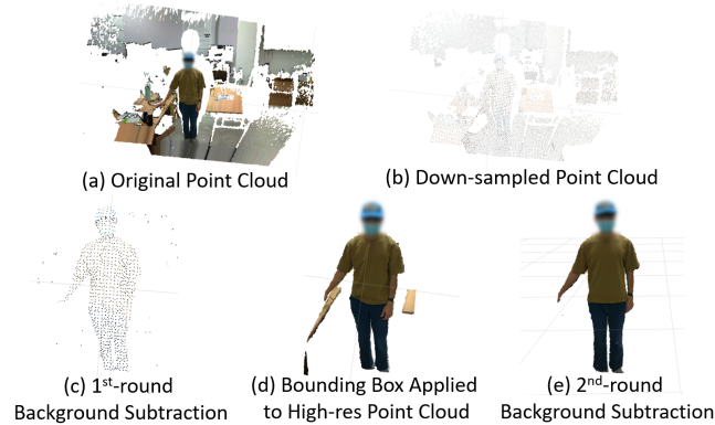
Figure 2: Visualization of the point cloud at each stage in the point cloud processing pipeline
