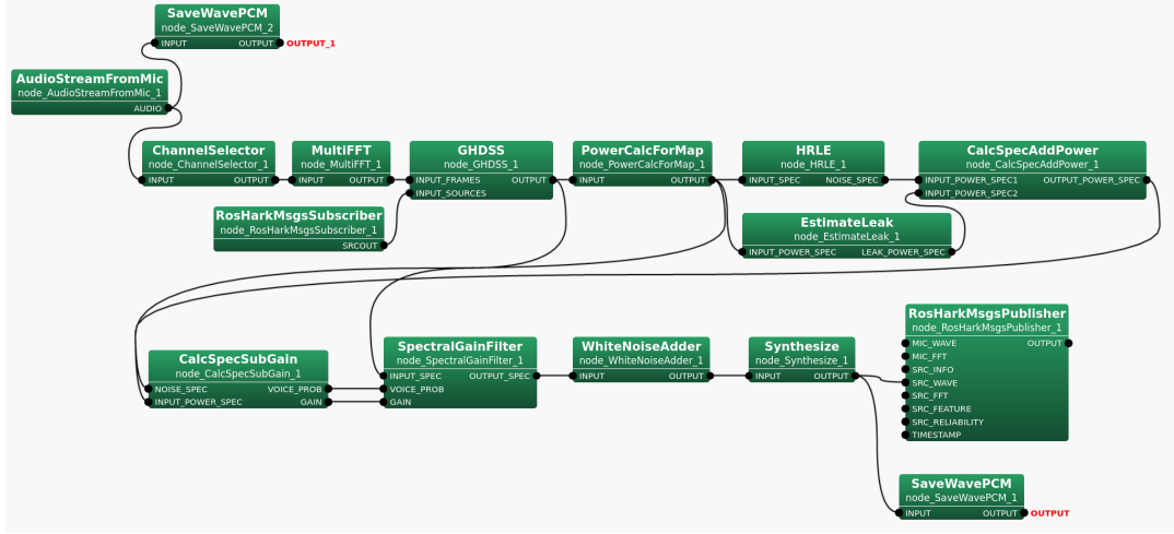
Figure 3: Depiction of the structure of the SSS pipeline
