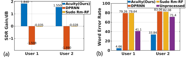
Figure 10: Audio Separation Results for Moving Subjects
