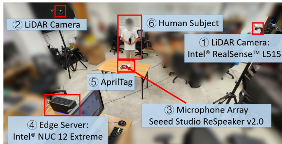
Figure 4: Experiment setup.
