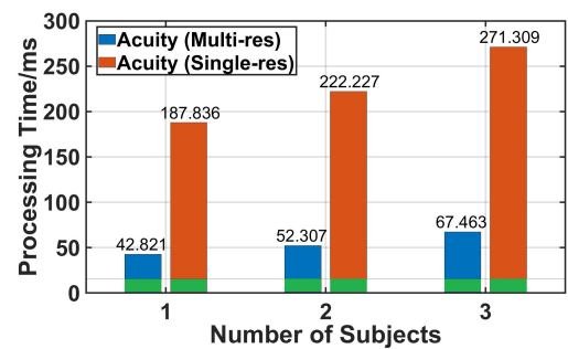
Figure 7: End-to-end latency of Acuity w/ and w/o multi-resolution pointcloud processing.
