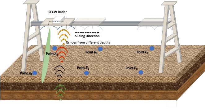
Fig. 1: Measurement campaign setup at WPI. A rail, holding the SFCW GPR, is placed between two ladders, with the GPR centrally positioned above two horizontal probe lines. Measurements were taken at 34, 57, and 79 inches above the ground. For each probe A_1 , A_2 , B_1 , B_2 , C_1 , and C_2 , SWC was recorded at 10, 20, 30, and 40 cm depths.
