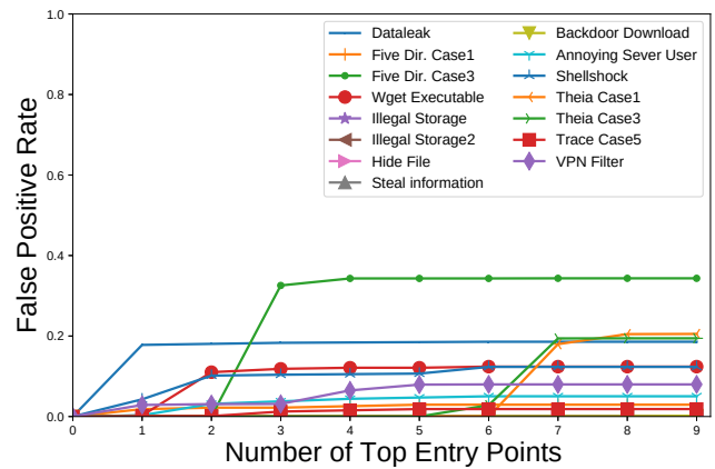
Figure 6: False positive using different number of top-ranked entry nodes
