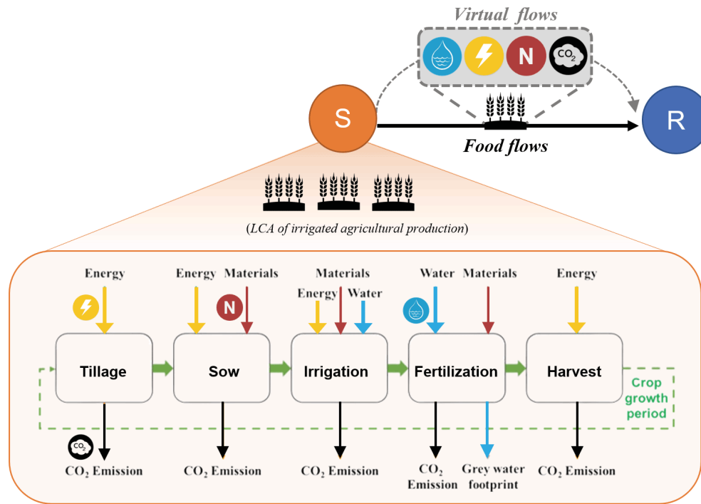
Fig. 5. An example of quantifying virtual flows of water, energy, nitrogen (N), and CO 2 embedded in food trade by using life cycle assessment (LCA) of irrigated agricultural production. S – sending system, R – receiving systems. The subplot of LCA is adapted from Xu et al. 2020b.
