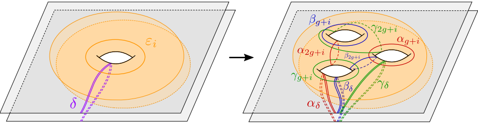
Figure 7: The local modification used to transform a Heegaard diagram (\delta, \epsilon) for a 3-manifold M into a trisection diagram (\alpha, \beta, \gamma) for the twist-spun manifold \mathcal{S}^*(M) .
