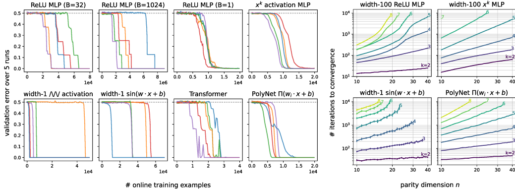
Figure 1: Main empirical findings at a glance. A variety of neural networks, with standard training and initialization, can solve the (n, k) -parity learning problem, with a number of iterations scaling as n^{O(k)} . Left : Training curves under various algorithmic choices (architecture, batch size, learning rate) on the (n = 50, k = 3) -parity problem. Right : Median convergence times for small (n, k) .
