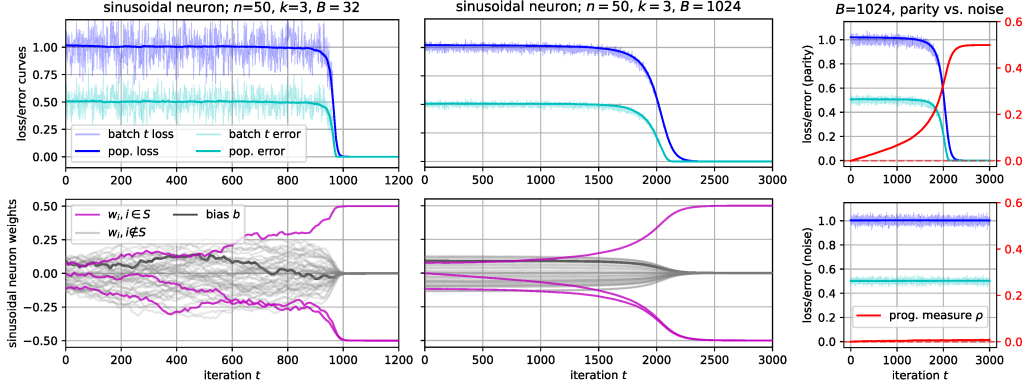
Figure 3: Hidden progress when learning parities with neural networks. Left, center : Black-box losses and accuracies exhibit a long plateau and sharp transition (top), hiding gradual progress in the SGD iterates (bottom). Right : A hidden progress measure which distinguishes gradual feature amplification (top) from training on noise (bottom).
