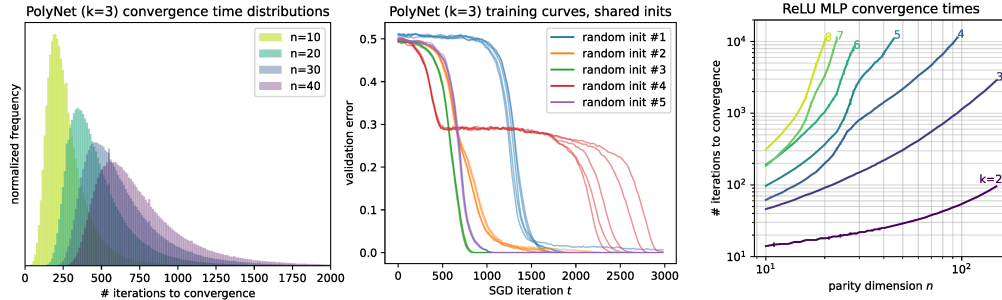
Figure 2: Black-box observations on the training dynamics. Left : Histograms of convergence times over 10^6 random trials, with heavy upper tails but no observed successes near t = 0 (unlike random search). Center : Loss curves (and thus, convergence time) depend heavily on initialization, not the randomness of SGD; B = 128, \eta = 0.01 are shown here. Right : The power-law exponent ( \alpha such that t_c \propto n^\alpha ) eventually worsens on larger problem instances.
