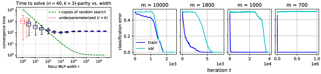
Figure 4: Parity as a sandbox for understanding the effects of model size and dataset size. Left : Success times vs. network width r on a fixed (40, 3) -parity task: in accordance with the theory, parallelization experiences diminishing returns (unlike expected success times for random search, shown in green). Underparameterized models ( r = 1, 2 ) were considered successful upon reaching 55% accuracy. Right : Training curves where only the sample size m is varied. The two center panels display “grokking”: a large gap between the time to zero train error vs. zero test error.
