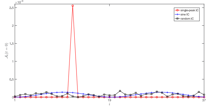
FIG. 1. Three types of initial conditions showing the distribution of initial amplitudes \mathcal{A}_i(t=0) in a system of N = 37 coupled oscillators. The red line with circle markers shows a single peak initial condition, the blue line with crosses shows a sine wave initial condition, and the black line with square markers shows a uniformly distributed random initial condition. In all three cases the Riemann sums pertaining to the three curves are equal.
