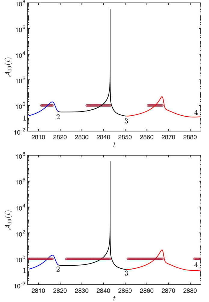
FIG. 9. Large amplitude events at i = 19 as seen in the right panel of Fig. 2 in the time domain shown superposed on locations where the precursor P identifies rapid growth (brown circles) due to the alignment of the trajectory with the stable direction of the saddle solution u_{\infty} (top panel) and of the v_{\infty} solution (bottom panel) of a single uncoupled oscillator.
