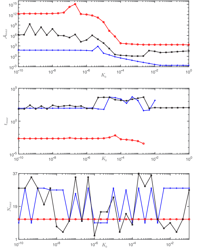
FIG. 11. Same as Fig. 6 but for the amplitude-dependent coupling (8). Red lines with circle markers show results for the single peak initial condition while blue lines with plus markers are the results for the sine wave initial condition. The top panel shows the variation in the maximum amplitude of observed excitations (on logarithmic scale) as a function of the coupling coefficient K_0 . The middle panel shows the variation in the time taken to reach the maximal excitation t_{\max} on logarithmic scale, also as a function of K_0 . Finally, the bottom panel shows the variation of the location N_{\max} of the maximal amplitude among the individual oscillators as a function of K_0 . Note that the single peak initial conditions were initialized at i = 12 .
