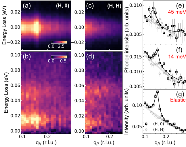
FIG. 3. Anisotropic momentum dependence of phonon intensity and dispersive CO excitations in \text{La}_{2-x}\text{Sr}_x\text{CuO}_4 ( x = 0.45 ). (a),(c) The elastic intensity map and (b),(d) the inelastic RIXS intensity map for visualizing the CO correlation and phonon branches along (H, 0) direction and (H, H) direction, respectively. (e)–(g) Integrated intensity for buckling phonon, acoustic phonon, and CO correlation, respectively, along both directions. Details of the fitting are presented in the Supplemental Material [18].
