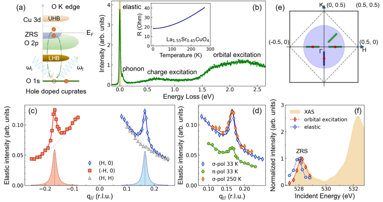
FIG. 1. Observation of charge order correlation by RIXS in overdoped metallic \text{La}_{2-x}\text{Sr}_x\text{CuO}_4 ( x = 0.45 ). The UHB and LHB refer to upper Hubbard band and lower Hubbard band, respectively. (a) Schematic plot of RIXS process at O K edge. (b) A typical RIXS spectrum at \mathbf{q}_{\parallel} = (0.12, 0) , displaying the elastic peak, phonon, charge, and orbital excitations. Inset: resistance curve displaying the metallic nature of the sample. (c) Integrated intensity of elastic peaks for positive and negative (H, 0) and (H, H) directions, using \sigma polarization. Red and blue curves are Lorentzian peak fits to the data with a polynomial background (gray dashed lines). (d) Polarization measurements with \sigma - and \pi -polarized light, collected at 33 and 250 K. (e) Reciprocal-space image. The blue shaded region is the accessible momentum-transfer range of O K edge. The green and blue lines indicate the momentum cuts, and red dots indicate the observed CO peaks. (f) XAS spectra near the ZRS absorption peak with \sigma polarization at normal incidence. Incident energy dependence of the integrated intensity of elastic peak and orbital excitation, normalized to the value at the ZRS peak.
