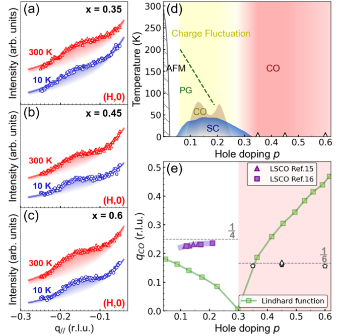
FIG. 4. Doping dependence of charge order correlation in overdoped \text{La}_{2-x}\text{Sr}_x\text{CuO}_4 (LSCO) and the extended phase diagram. (a)–(c) CO peak profiles measured by Cu L edge REIXS in LSCO with x = 0.35, 0.45, 0.6 , respectively. The offset is applied for clarity. L is fixed at 1.1 r.l.u. The peak is nearly temperature independent up to 300 K. (d) The extended CO phase diagram of cuprates. It shows superconducting dome defined by T_c , antiferromagnetism (AFM) defined by T_N [44], pseudogap determined from the Nernst coefficient [45], underdoped charge order and charge fluctuation [16,35,46], and overdoped charge order. (e) The doping dependence of the CO wave vector in LSCO and nesting vector obtained from Lindhard function.
