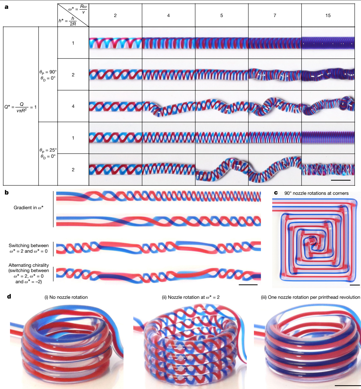
Fig. 2 | Patterning geometric complexity across scales. PDMS filaments extruded from shell–fan-core nozzles presented in Fig. 1b and Extended Data Fig. 1. a , Filaments printed at varying values of \omega^* , h^* and \theta_p (with constant \theta_D = 0^\circ and Q^* = 1 ). b , Patterning 1D filaments with gradients in \omega^* (rows 1 and 2), switching in \omega^* (row 3) and alternating chirality (row 4). Print parameters were \theta_p = 25^\circ , \theta_D = 0^\circ , Q^* = 1 , h^* = 1 , v = 2 \text{ mm s}^{-1} . c , A 2D square spiral pattern with 90^\circ
