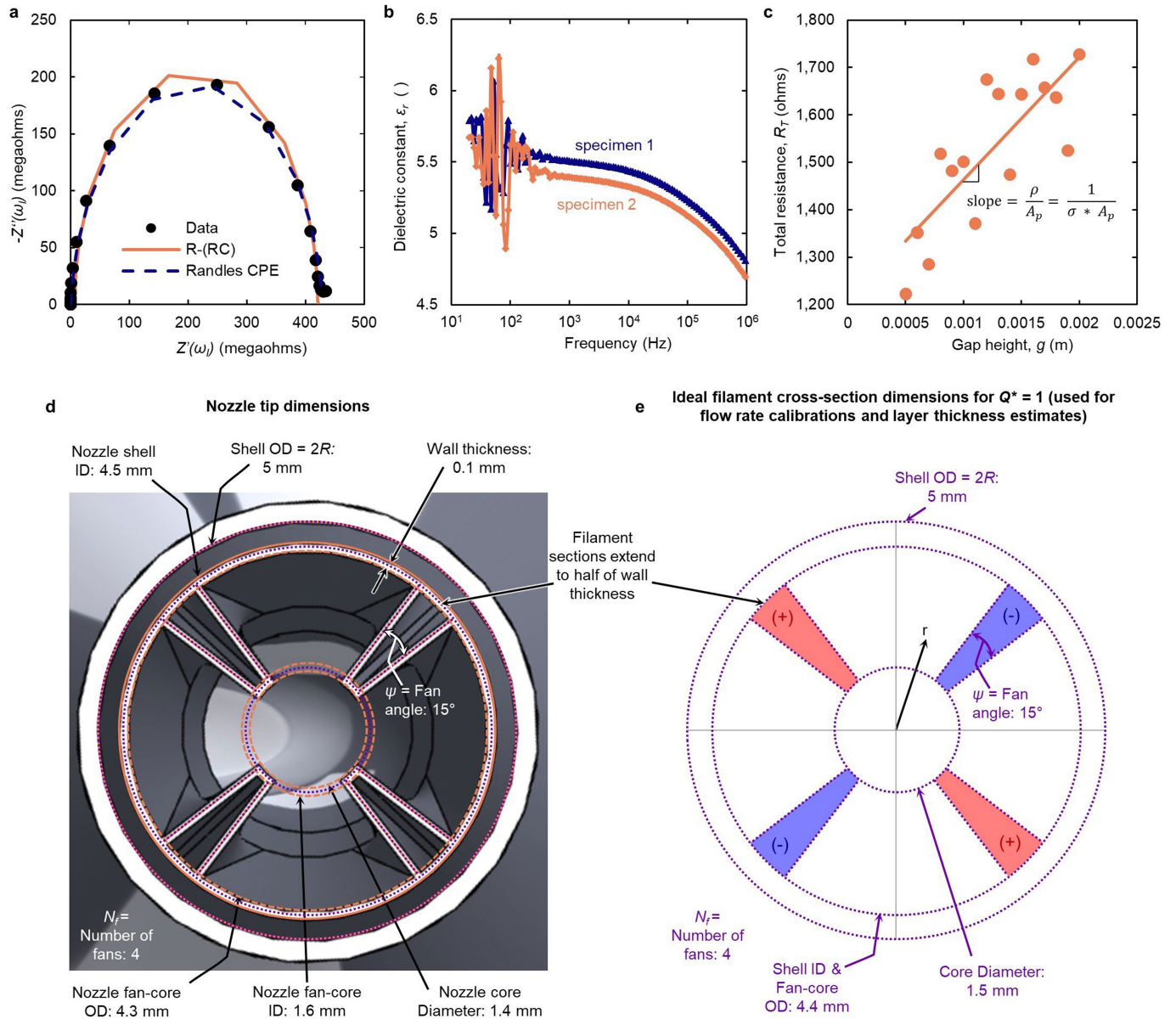
Extended Data Fig. 5 | Material properties and nozzle geometry for HDEA filaments. a, b , Dielectric constant of crosslinked dielectric elastomer ink. a , Static dielectric constant measurements. A Randles CPE model was found to fit the data better than a resistor in series with a parallel resistor and capacitor (R-(RC)). b , Dynamic dielectric constant for two specimens. For each specimen, capacitance measurements were performed three times. The plotted data points represent the average dielectric constant computed from the three measurements. For the tested capacitance, low-frequency measurements are expected to be of low accuracy owing to device signal noise. c , Conductivity measurement of carbon-black-based conductive electrode ink. Plot of total resistance, R_T , versus gap height, g , using an AC signal frequency of 1 kHz.
