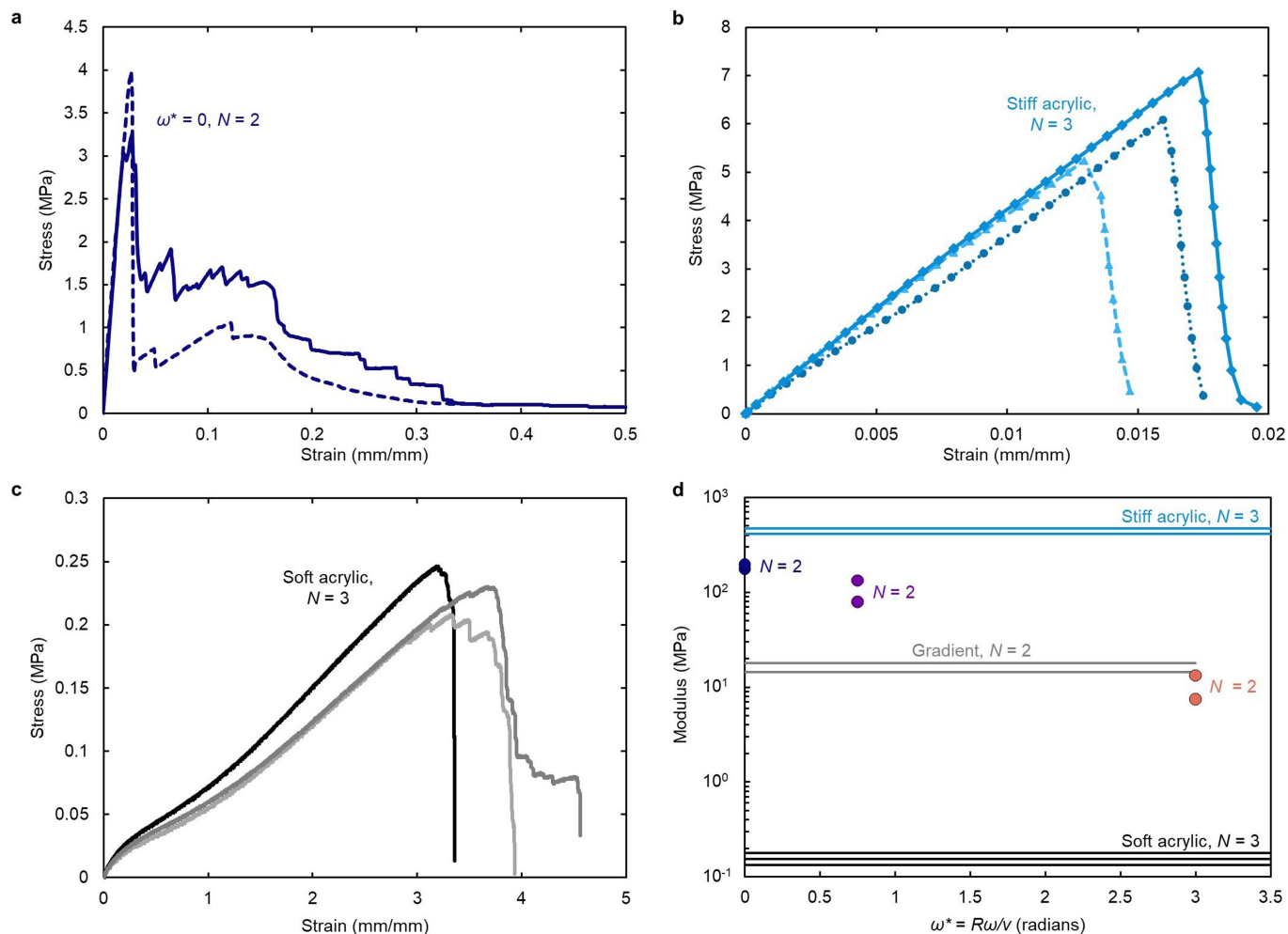
Extended Data Fig. 10 | Tensile measurements on 3D lattices. a–c, Stress–strain curves for springy lattices composed of filaments with \omega^* = 0 ( N = 2 ) ( a ), lattices composed of only stiff acrylic filaments ( N = 3 ) ( b ) and lattices composed of only soft acrylic filaments ( N = 3 ) ( c ). d, Moduli of springy lattices as a function of \omega^* ( N = 2 for each \omega^* ). Solid grey lines are the moduli of the
