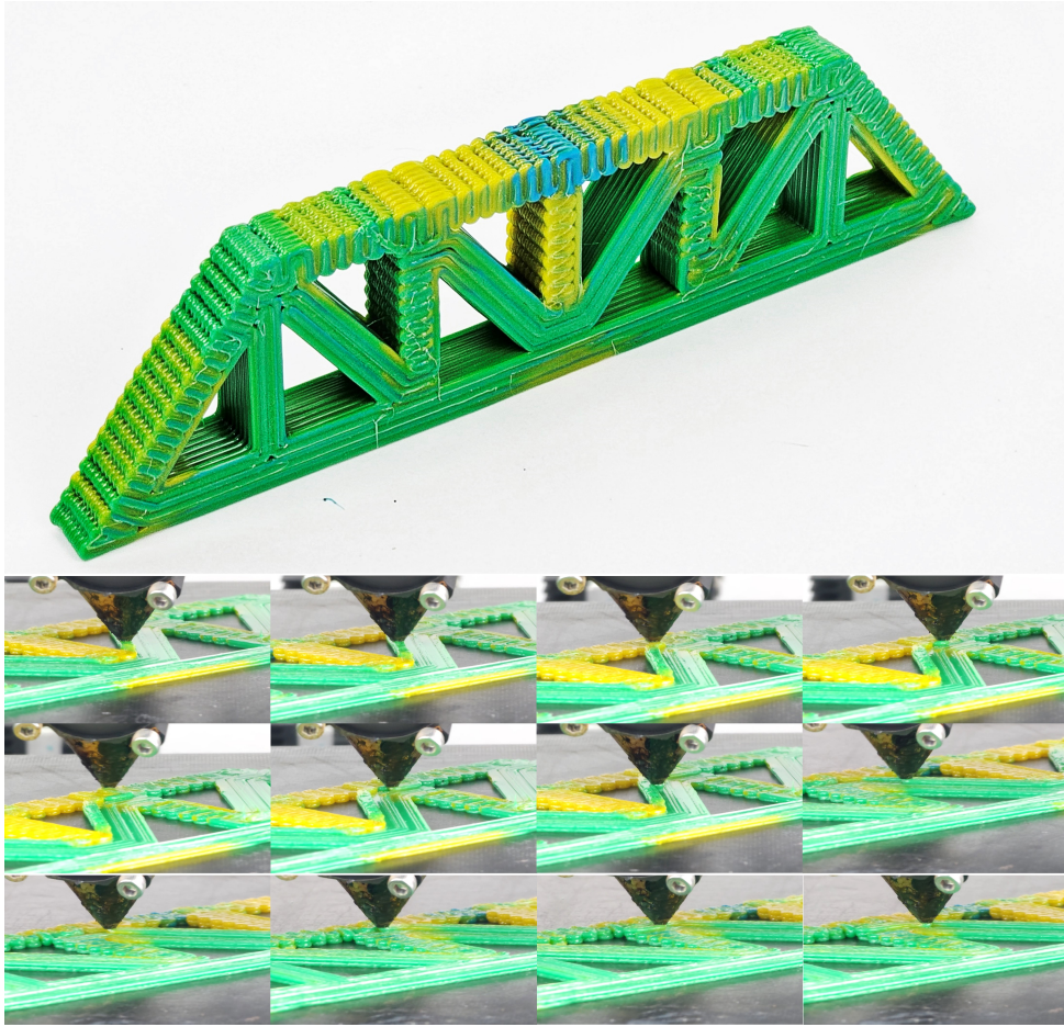
Figure 3: Upper: Printed Pratt truss with three different filaments: yellow PLA Filament, green PLA Filament and blue PLA Filament. Lower: the three-filament continuous printing process.
