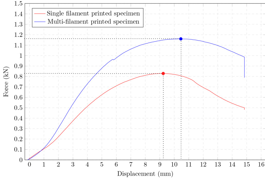
Figure 5: Result of three-point bending test
