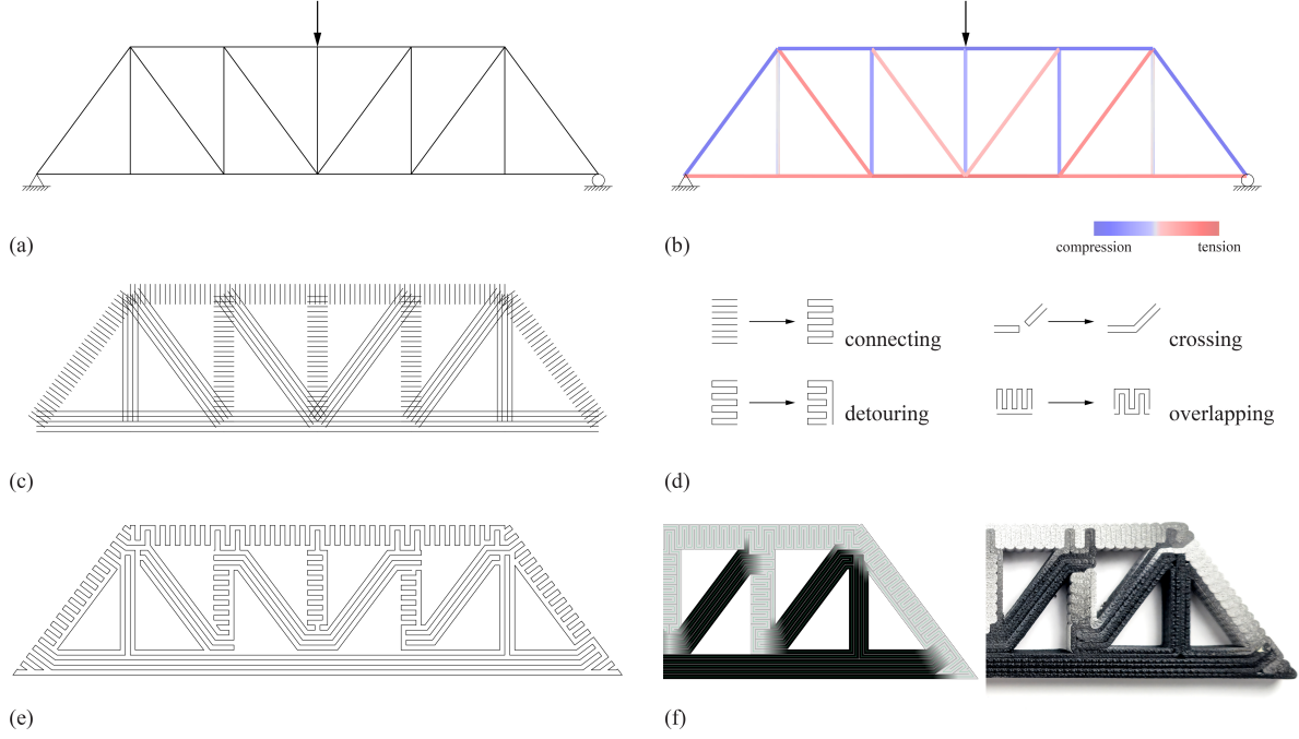
Figure 1: Multi-material printed truss toolpath generation process: (a) Input curves; (b) axial force conditions solved by Karamba3D; (c) raw curves according to the axial forces; (d) post-processing methods to form a continuous toolpath; (e) the final toolpath; (f) left: multi-material visualization of the print, right: multi-material printing
