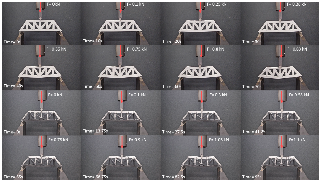
Figure 6: Three-point bending test of two PLA truss specimens. Upper two rows: single material (Regular white PLA) printed controlled sample. Lower two rows: Multi-material (Regular white PLA and carbon fiber enforced black PLA) printed experimental sample.
