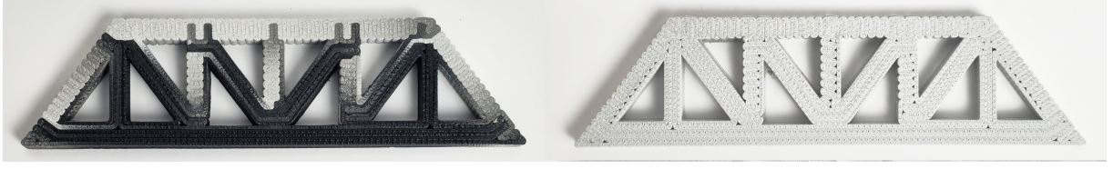
Figure 4: Two samples for three-point bending test. Left: multi-material experimental specimen printed with HATCHBOX white PLA and OVERTURE Carbon Fiber reinforced PLA. Right: single material control group specimen printed with HATCHBOX white PLA only.
