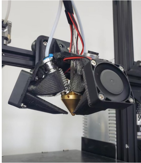
Figure 2: 3-in-1-out nozzle designed for Multi-material (filament) printing
