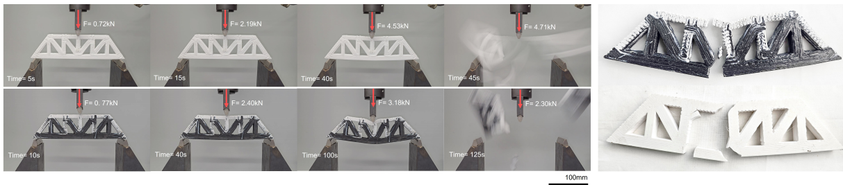
Figure 7: Left: three-point bending test for examining structure's fracture behavior. Upper left row: single material (Regular white PETG) printed controlled sample. Lower left row: Multi-material (Regular white PETG and carbon fiber enforced black PETG)printed experimental sample. Right: A comparison between the post-test multi-material and single-material samples. Upper right image:multi-material specimen, Lower right image:single-material specimen
