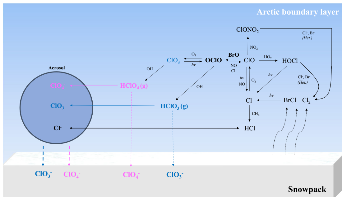
Fig. 3 | Atmospheric formation and the fate of \text{HClO}_3 and \text{HClO}_4 . Simplified diagram of the proposed potential formation mechanism of gas-phase \text{HClO}_3 (blue) and \text{HClO}_4 (pink) in the Arctic boundary layer during springtime after polar sunrise. The produced \text{HClO}_3 and \text{HClO}_4 can be taken up by the surface of aerosols and converted into \text{ClO}_3^- and \text{ClO}_4^- , respectively. The deposition of aerosols and/or the
