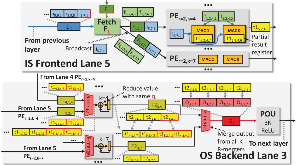
Fig. 11: ISOSceles IS frontend and OS backend.
