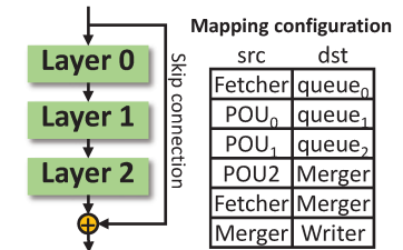
Fig. 13: Mapping ResNet block to ISOSceles.
