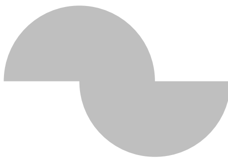
Figure 2. A set that is star-shaped but not effectively star-shaped.
