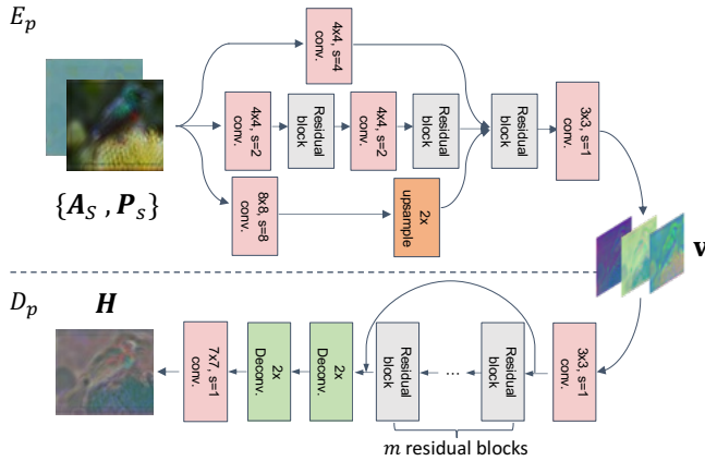
Fig. 4. Multi-scale encoder E_p and residual decoder D_p . Within the encoder E_p , multiple branches are designed for enabling better feature extraction and more efficient backward gradient flow.
