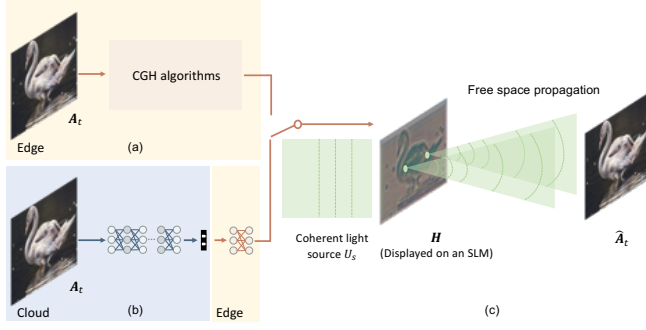
Fig. 2. A simplified illustration for the cloud-edge collaborative holographic displaying model. Prevalent solutions mainly adopt the strategy shown in (a), where the phase data is computed at the edge side, while the proposed framework enables a collaborative cloud-edge displaying solution, as shown in (b). (c) shows a simplified holographic display model. When illuminated by the coherent light source U_s , the spatial light modulator (SLM) modulates the phase of the light wave according to the hologram H . The modulated light wave arrives at the target plane after propagating in space. The content perceived by human eyes (or captured by cameras) is mainly from the intensity of the complex wave field, i.e. , mainly from the amplitude \hat{A}_t .
