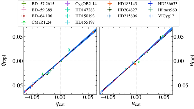
Fig. 5. Weighted mean values of Stokes parameters of high-polarization standards as measured by RoboPol vs. catalogue values from Table 1. The black dashed line is y = x the red solid line is the ordinary least squares regression fit to the data. The light blue region is the 1\sigma uncertainty region of the fit.
