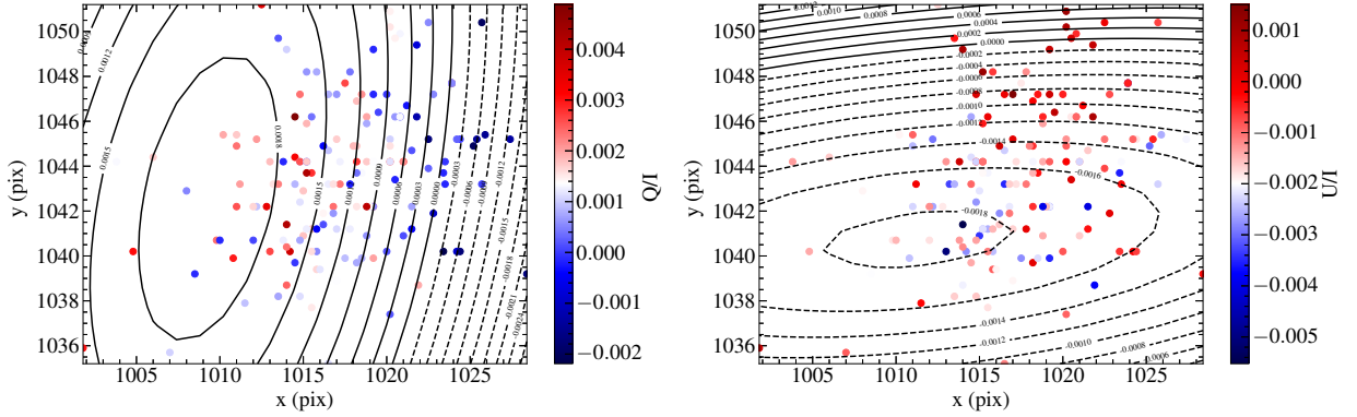
Fig. 3. Relative Stokes parameters of zero-polarization standards from Table 1 observed in 2019 in the central masked area as a function of the position on the CCD. Color of points indicates the deviation of Q/I or U/I from zero. The planar contours show the fitted quadratic surface.
