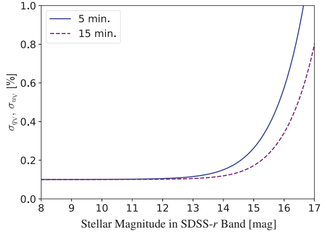
Fig. A.3: Uncertainties on individual measurements of the relative Stokes parameters in SDSS-r band as a function of star's magnitude as expected from PASIPHAE's northern instruments (WALOP-N) for 5 minutes and 15 minutes exposure times shown with solid blue and dashed purple lines, respectively.
