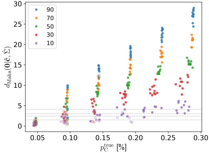
Fig. 10. Significance of the cloud detection ( d_{\text{Maha}}(\mathbf{0}|\hat{\mathbf{c}}, \hat{\mathbf{\Sigma}}) ) as a function of the input cloud polarization and for the several f_{\text{bg}} values corresponding to the same reconstructions characterized through Fig. 9. The horizontal lines indicate threshold values corresponding to detection levels with 68%, 95%, 99%, and 99.98% probabilities of finding a distance lower than threshold. Symbol and color conventions are the same as in Fig. 9.
