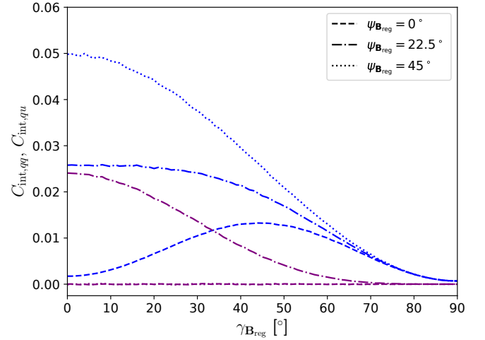
Fig. B.4: Dependence of C_{\text{int},qq} (blue) and C_{\text{int},qu} (purple) as a function of \gamma_{\mathbf{B},\text{reg}} and for three values of the position angles: \psi_{\mathbf{B},\text{reg}} = 0^\circ (dashed lines), \psi_{\mathbf{B},\text{reg}} = 22.5^\circ (dashed-dotted lines), and \psi_{\mathbf{B},\text{reg}} = 45^\circ (dotted lines). A value of A_{\text{turb}} = 0.2 is chosen here. The elements of the covariance matrix are given in units of P_{\max}^2 . A value of 0.01 corresponds to a polarization uncertainty ( \sigma_q or \sigma_u ) of 10 per cent of P_{\max} .
