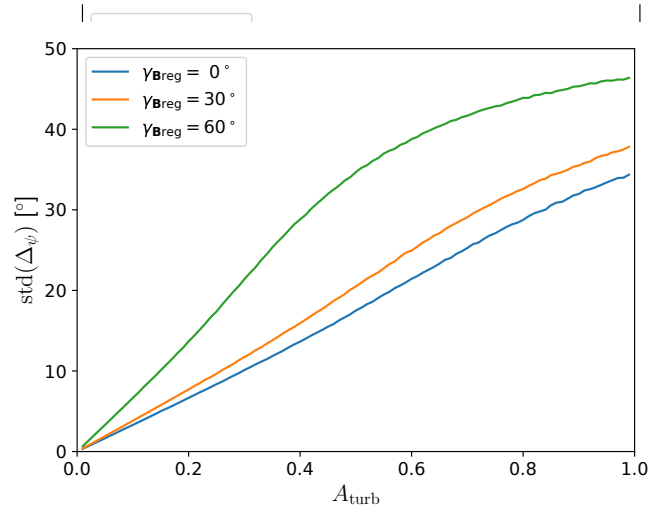
Fig. B.2: Scatter in EVPA as a function of A_{\text{turb}} . For each value of A_{\text{turb}} , 10^5 realizations of \mathbf{B}_{\text{tot}} are computed. The Stokes parameters are computed and polarization position angles determined and compared to the polarization vector corresponding to the regular component only. The standard deviation of the polarization angle difference is then computed and plotted against A_{\text{turb}} . We carry the analysis for \gamma_{\text{Breg}} = 0^\circ, 30^\circ and 60^\circ .
