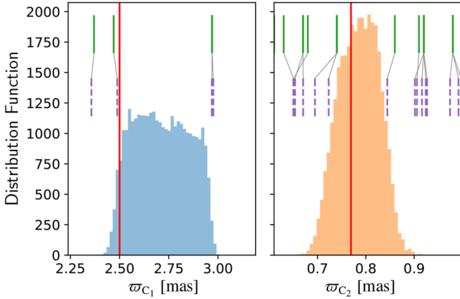
Fig. 7. Estimated posterior distributions for w_{C1} (left) and w_{C2} (right) in [mas] with marked observed and input parallaxes of surrounding stars with (dashed) purple and (continuous) green vertical segments, respectively, similar to Fig. 4. Vertical red lines indicate the input parallaxes of the clouds. As before, some stars with very similar (true) parallaxes (green) are dispersed after randomization.
