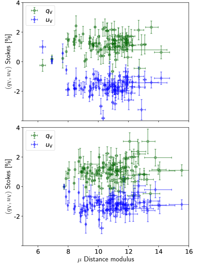
Fig. 14. (q_V, u_V) - \mu plane for the polarization data in Panopoulou et al. (2019b). Top and bottom panels correspond to their 1-cloud and 2-cloud regions, respectively. The relative Stokes parameters q_V 's are shown by dark green circles and the u_V 's are shown by blue diamonds. Vertical and horizontal errorbars show the 68% confidence level on measurements on polarization and distance modulus, respectively. For visualization purposes we omit to show two stars at distance modulus 1.6 and 18.6 in the 1-cloud region.
