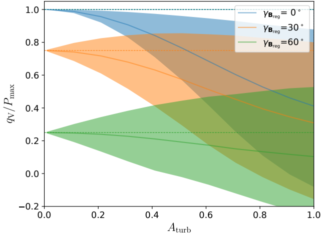
Fig. B.3: Distributions of q_V/P_{\max} corresponding to various inclination angle and amplitude of the intrinsic scatter. We carry the analysis out for \gamma_{\mathbf{B},\text{reg}} = 0^\circ, 30^\circ , and 60^\circ and A_{\text{turb}} \in [0, 1] . For each value pair, 10^5 realizations of \mathbf{B}_{\text{tot}} are computed and q_V is evaluated. The continuous lines show the mean of the distribution for \gamma_{\mathbf{B},\text{reg}} = 0^\circ, 30^\circ , and 60^\circ in blue, orange and green, respectively. The shaded areas indicate the range span between percentiles 16 and 84 of the distribution. The dashed lines indicate the q_V/P_{\max} values obtained when no stochastic term is added in the magnetic field.
