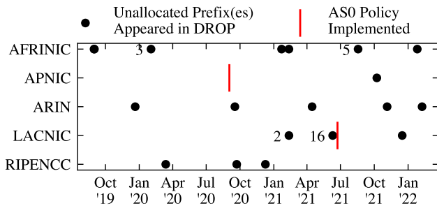
Figure 6: Timeline of when address space unallocated by RIRs appeared on DROP, and when an AS0 policy was implemented by an RIR. In practice, the ability of an attacker to hijack an unallocated prefix is not affected by the RIRs' current AS0 policies.
