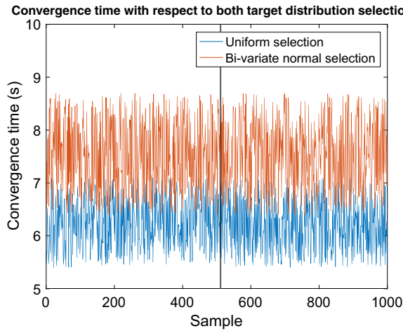
Fig. 8 Convergence times of 1000 tests on the experimental setup with respect to both distribution selections. Uniform selections of targets are simpler to be handled by the optimal target assignment because of the availability of the more pairing options between astrobots and targets. The faster convergences of this selection class are shown in the figure. Nevertheless, the applied bi-variate normal selections' convergence times are noticeably comparable with those of the uniform selections. Given the fact that target assignments and coordination under bi-variate normal selections are more challenging, we conclude that CSA is efficient under various potential distributions of targets
