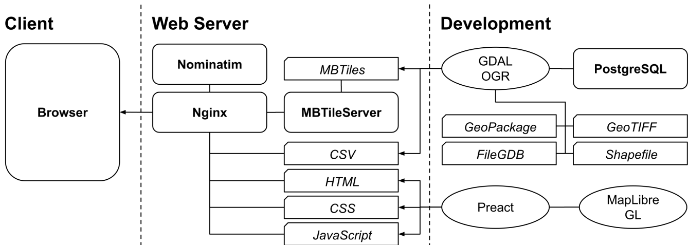
Figure 2: Diagram of the Master Plan Data Viewer architecture.
