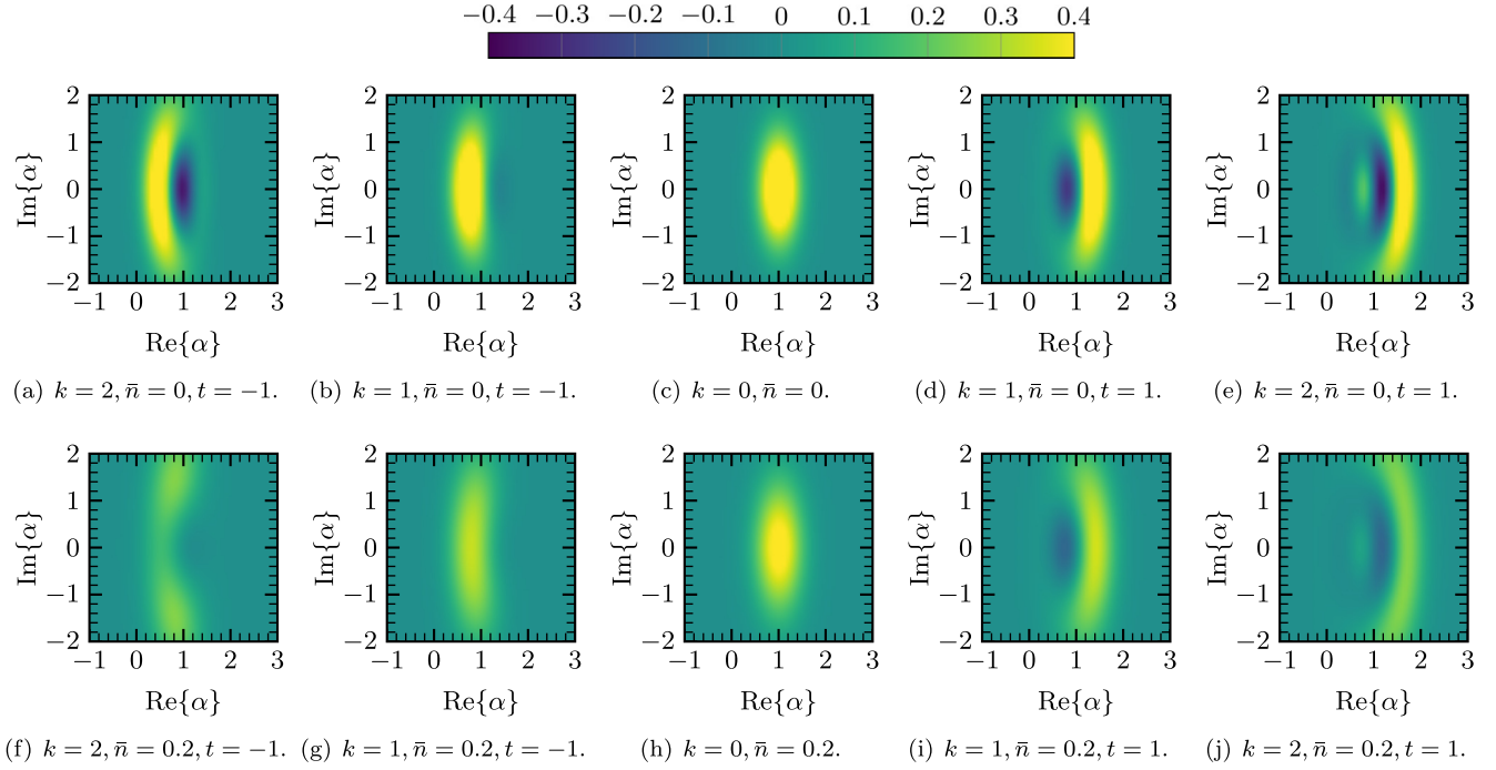
FIG. 3. Wigner W function W(\alpha) of \Xi_{\eta}^{(k)} for different values of k and \bar{n} with \mu = 1 , \phi = 0 , and r = -0.5 .
