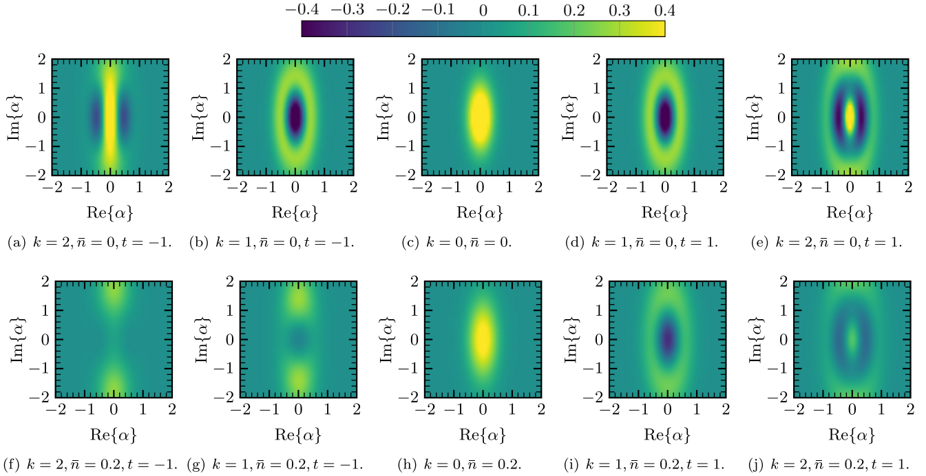
FIG. 2. Wigner W function W(\alpha) of \Xi_{\eta}^{(k)} for different values of k and \bar{n} with \mu = 0 , \phi = 0 , and r = -0.5 .
