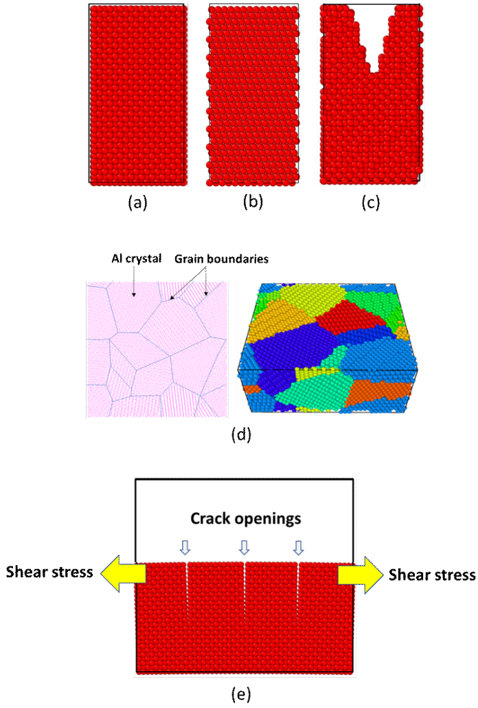
Fig. 2. Models for oxidation simulation. (a) Al(1 0 0) crystal with no defects, (b) Al(1 1 1) crystal with no defects, (c) model with surface scratch, (d) grain boundary model and (e) microcrack model
