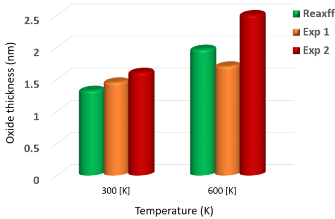
Fig. 3. Comparison of the growth of the oxide film with temperature increase in the ReaxFF and experiment
