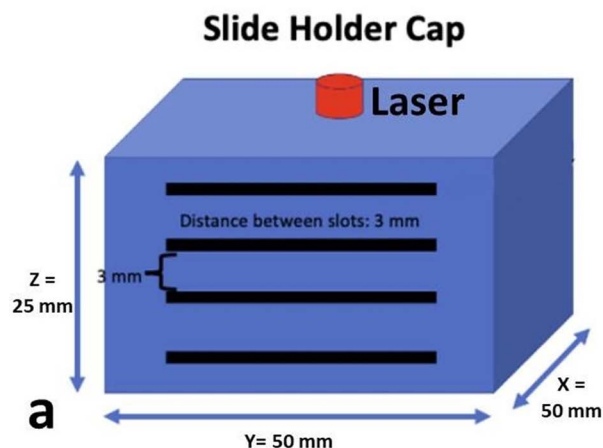
Fig 11. Microscope with variable magnification. (a) A 3D-printed cap with 40-mm-wide \times 2-mm-high slots to receive standard glass microscope slides. A matching set of slots on the opposite side allowed a slide to be passed through the cap in the X direction. Because the magnification increases with the sample-to-image sensor distance, the slots allowed the user to select discrete magnifications. (b) Modified cap attached to the holographic microscope.
