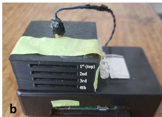
Fig 11. Microscope with variable magnification. (a) A 3D-printed cap with 40-mm-wide \times 2-mm-high slots to receive standard glass microscope slides. A matching set of slots on the opposite side allowed a slide to be passed through the cap in the X direction. Because the magnification increases with the sample-to-image sensor distance, the slots allowed the user to select discrete magnifications. (b) Modified cap attached to the holographic microscope.
