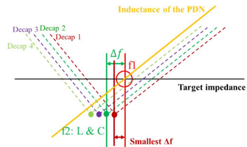
Fig. 4. Example for the poles and zeros algorithm
