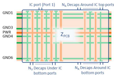
Fig. 3. Impedance matrix for PDN optimization [9].
