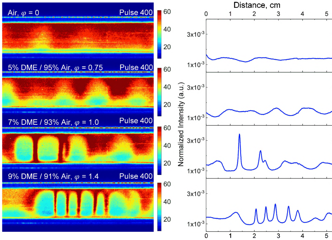
Figure 9: Left: single-shot ICCD images of nanosecond pulse discharges in DME-air mixtures at different equivalence ratios (labeled above each image) at pulse 400. The initial temperature is 300 K. The pulse frequency is 10 kHz. The camera gate is 500 ns for emissions within the pulse (“Discharge On”). Units in colorbars are arbitrary units (a.u.). Right: Normalized intensity distribution along the stream-wise direction (averaged between the discharge gap).
