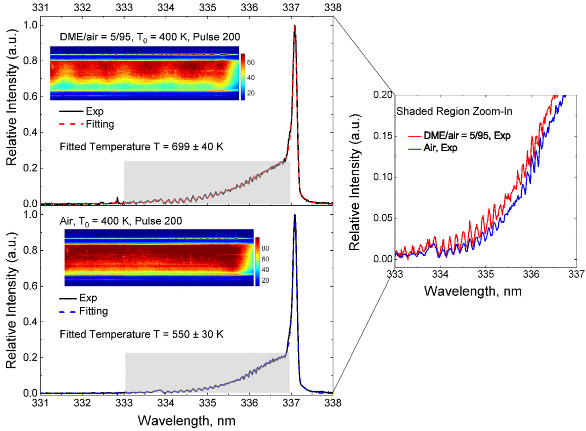
Figure 6: Left: Comparisons of experimental and synthetic N_2 emission spectra (second positive band system) of the air and DME-air plasmas at pulse 200. Right: The zoom-in plot of the shaded regions of the spectrum.
