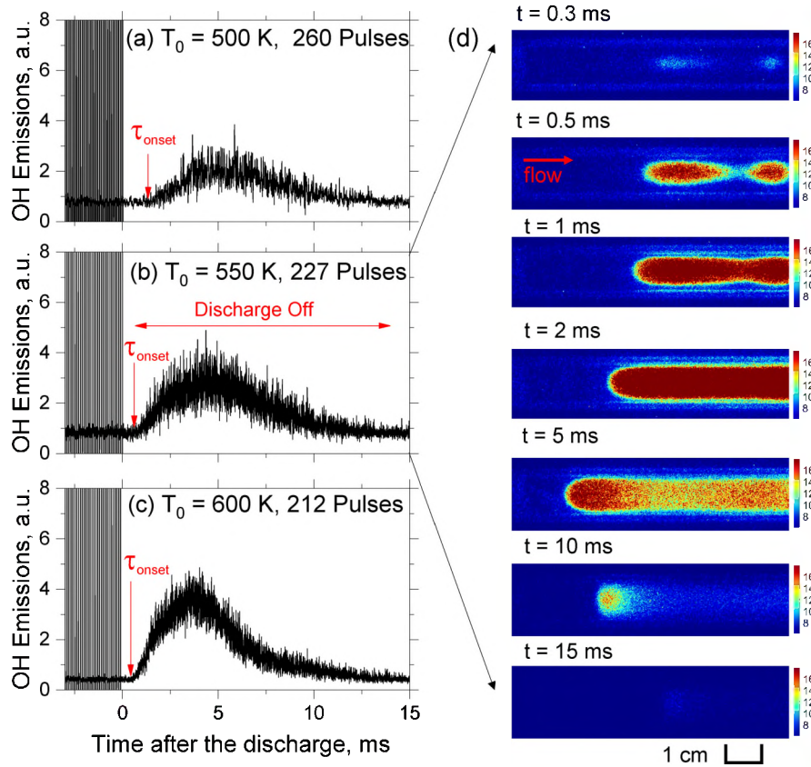
Figure 3: Left (a,b,c): Time-resolved UV emission (310 nm) from a 5% DME/air mixture during ignition by a repetitive nanosecond pulsed discharge burst. Red arrows indicate the time when OH emissions start to rise (OH onset time). The initial temperature T_0 = 500, 550 , and 600 K. P = 100 Torr. \nu = 10 kHz. Right (d): ICCD camera images of the flame propagation. Units in colorbars are arbitrary units (a.u.). The flow direction is labeled. T_0 = 550 K.
