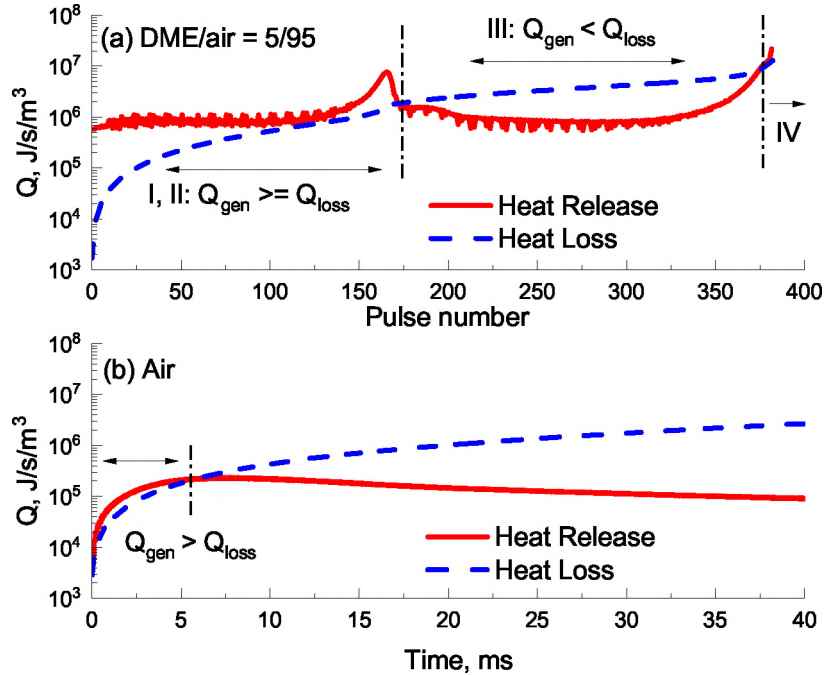
Figure 7: The order of magnitude estimation for \dot{Q}_{gen} and heat loss \dot{Q}_{loss} (both defined in the text) for the (a) DME/air = 5/95 and (b) air mixture. Stage I - IV in (a) are discussed in the text. Note: heat release rate is running-averaged for every pulse.
