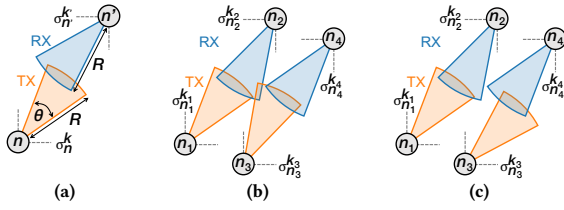
Figure 3: (a) A feasible link \ell = (\sigma_n^k, \sigma_{n'}^{k'}) , (b) A secondary interfering TX sector \sigma_{n_3}^{k_3} to RX sector \sigma_{n_2}^{k'_2} , (c) The secondary TX interference in (b) can be avoided by steering node 3's TX beam in \sigma_{n_3}^{k_3} , so that both links (\sigma_{n_1}^{k_1}, \sigma_{n_2}^{k'_2}) and (\sigma_{n_3}^{k_3}, \sigma_{n_4}^{k'_4}) can be simultaneously activated.
