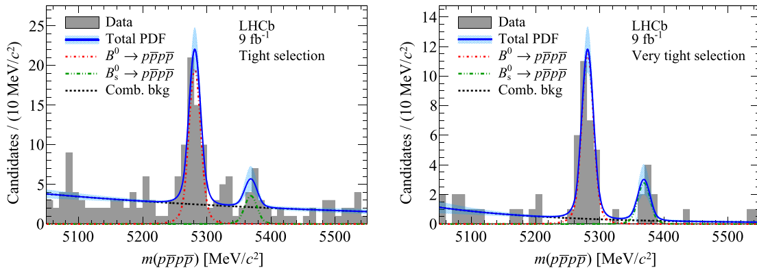
FIG. 1. Combined Run 1 plus Run 2 invariant-mass distributions of B^0_{(s)} \rightarrow p\bar{p}p\bar{p} candidates satisfying (left) the tight and (right) the very tight selection criteria discussed in the text. The fit results (solid blue lines) for these samples are shown together with the fit model components. The hashed cyan band corresponds to the 1\sigma model uncertainty based on the fit covariance matrix.
